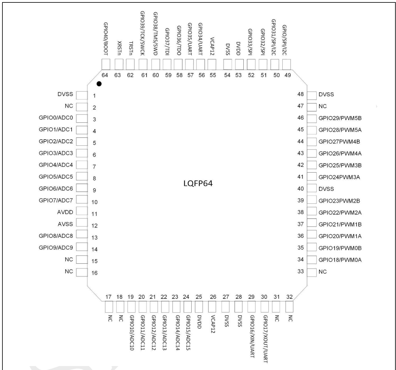
图 3-3: SPC1168 LQFP64 引脚排列
