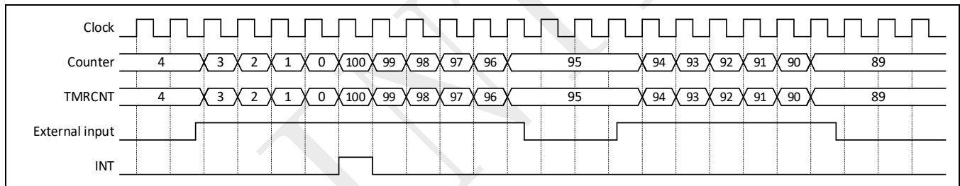
Figure 6-3: Timer waveform in gated timer mode (TMRLOAD=100)
