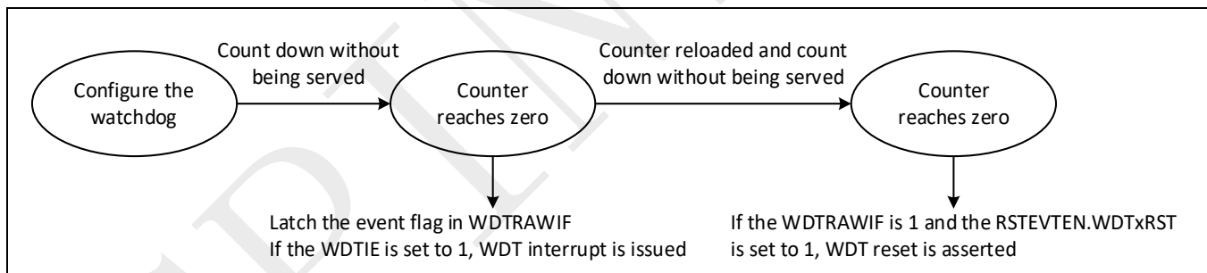
Figure 7-1: Watchdog operation flow
