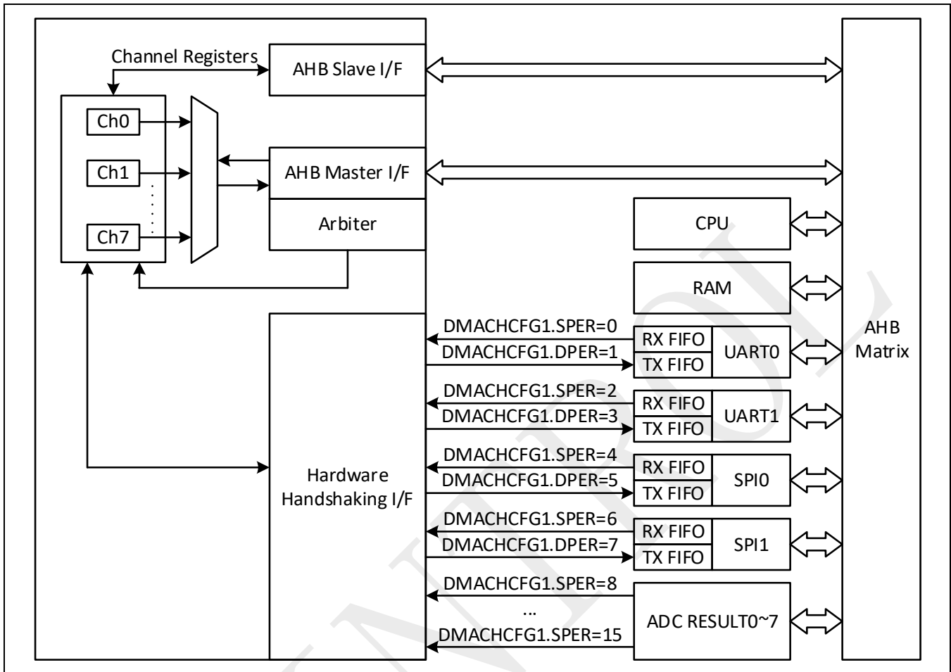
Figure 26-1: DMA block diagram
