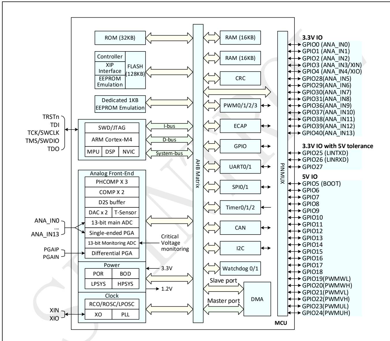
Figure 1-1: Block diagram of SPC1169
