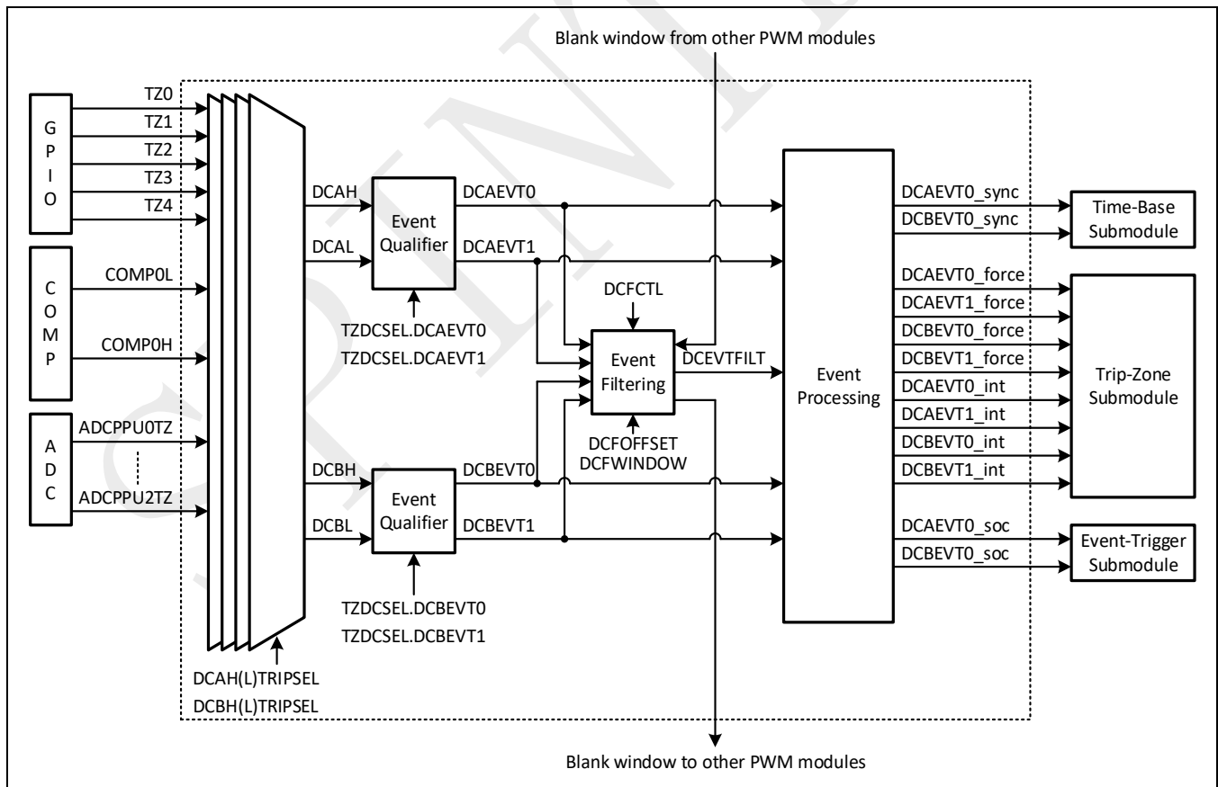
Figure 8-16: Digital Compare sub-module structure
