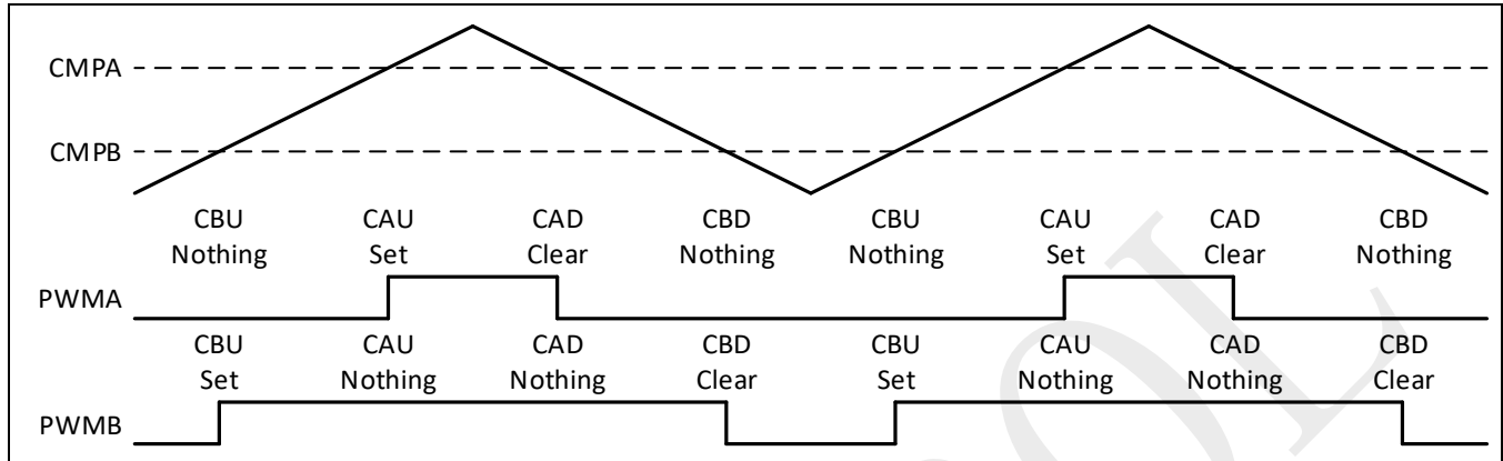
Figure 8-9: Up-Down-Count, dual edge symmetric waveform of Action-Qualifier
