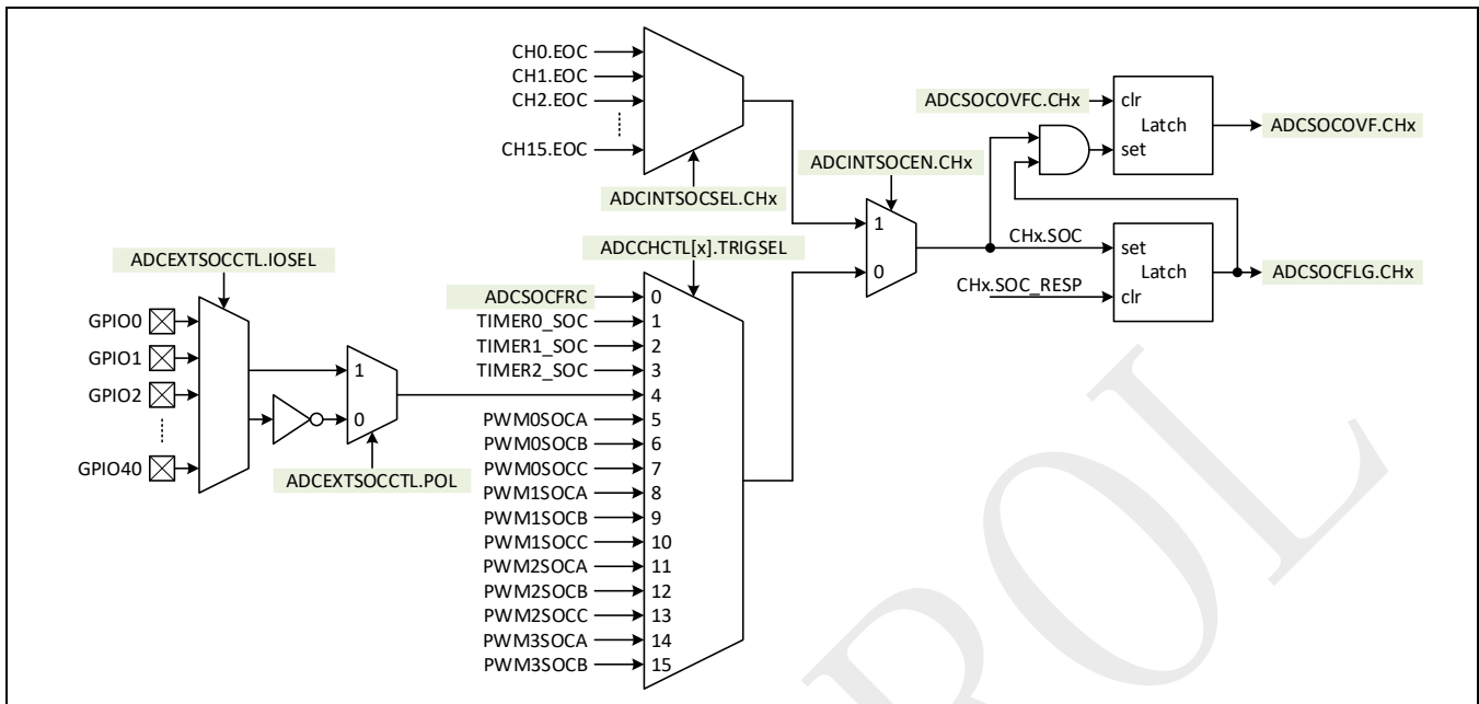
Figure 10-2: ADC Channel SOC generation
