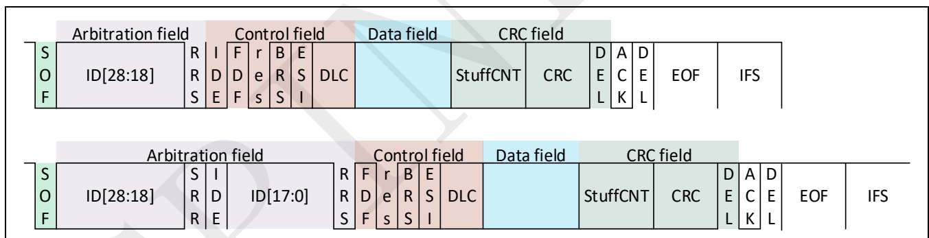
Figure 22-4: ISO FDCAN frame format
