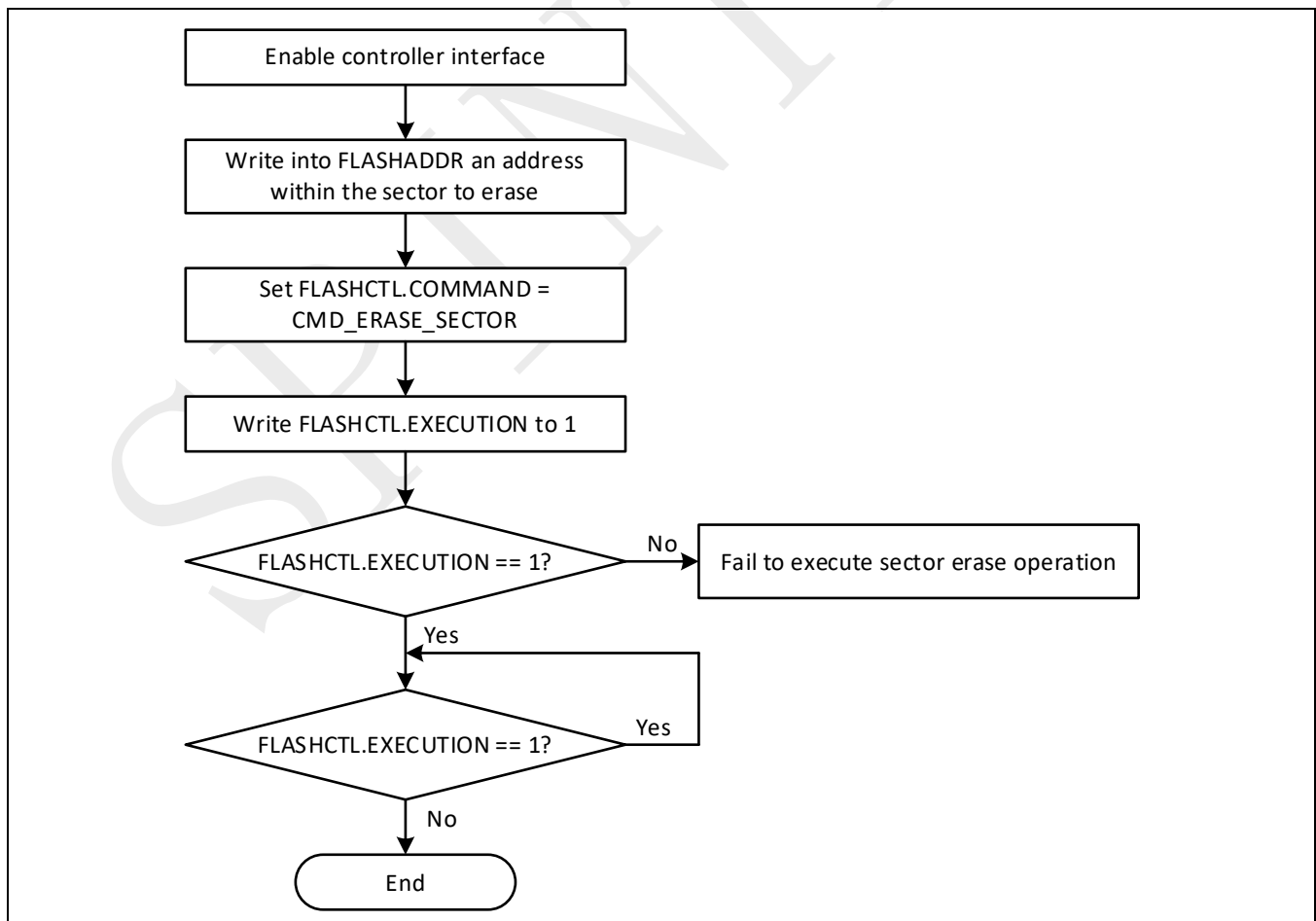
Figure 24-5: Flash memory Sector Erase procedure
