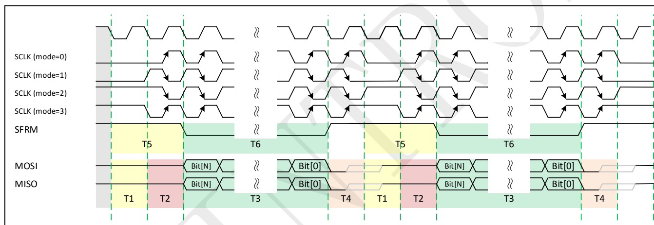
Figure 20-10: PSP protocol (Consecutive Transfers)
