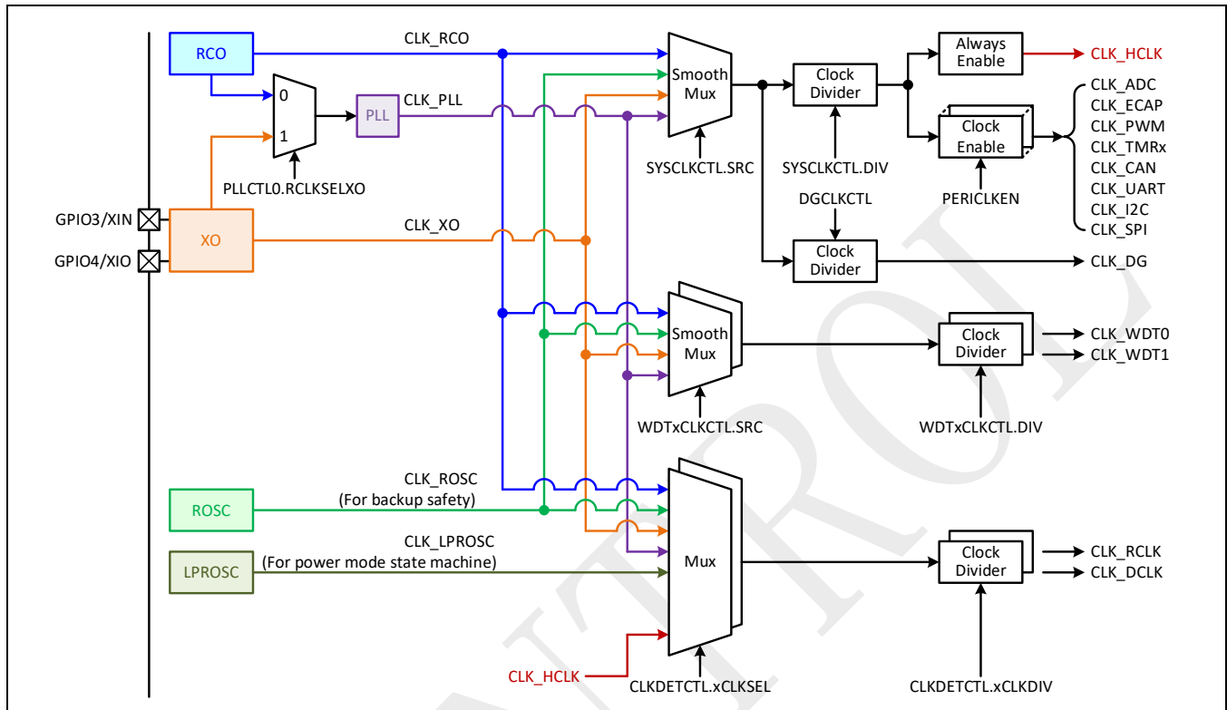
Figure 1-2: SPC1169 clock tree
