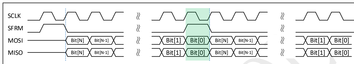
Figure 20-8: SSP protocol (back to back transfer)
