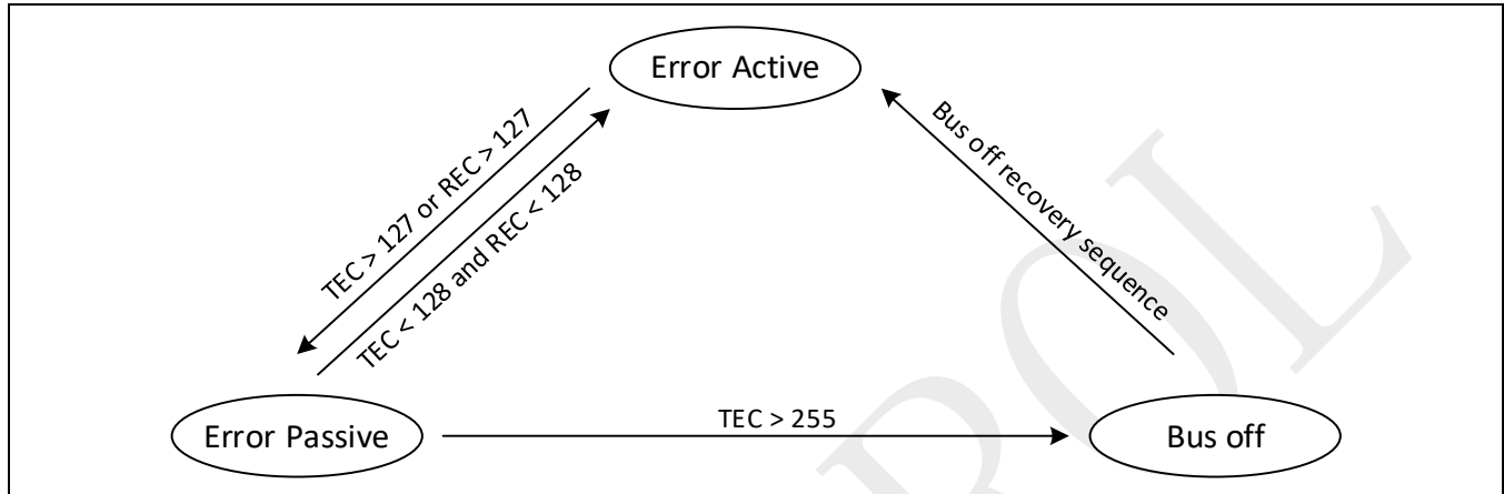
Figure 22-8: CAN node error state conversion
