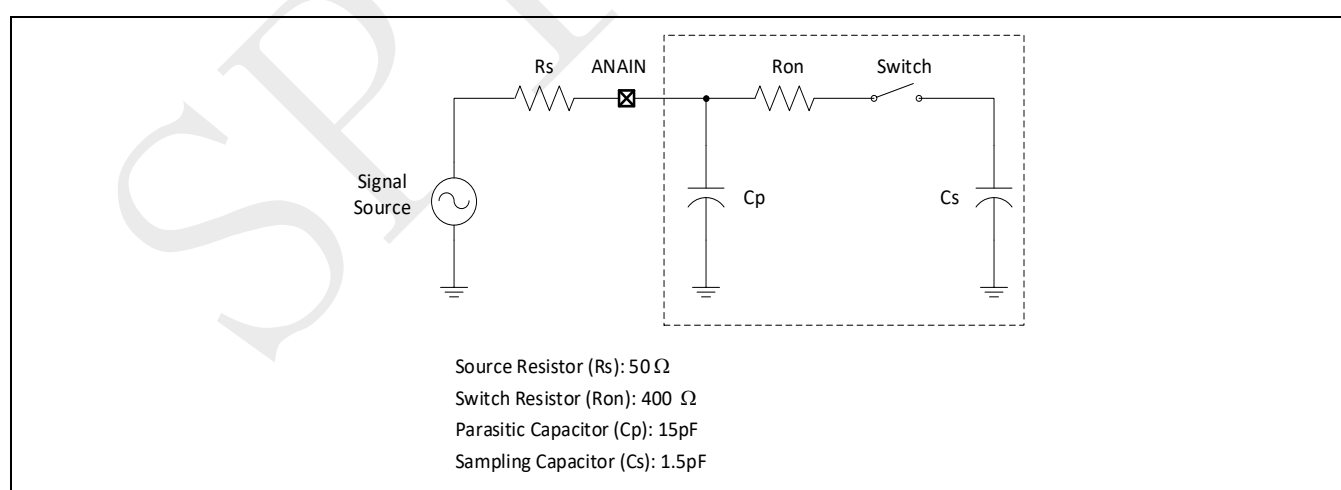
Figure 10-3: Analog input pin model
