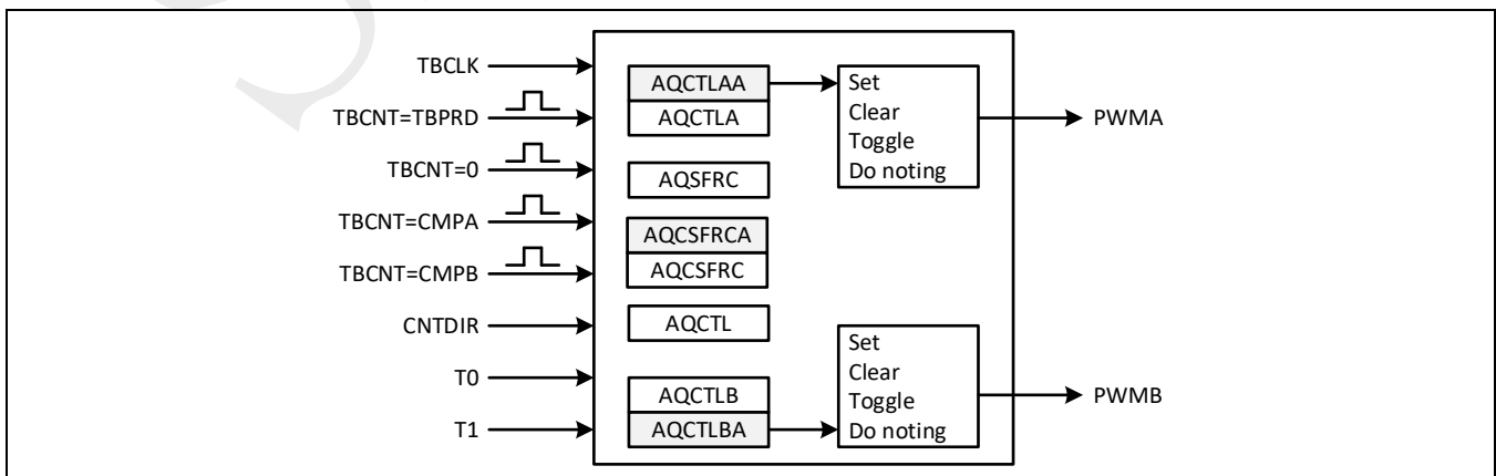
Figure 8-8: Action-Qualifier sub-module inputs and outputs
