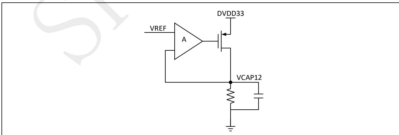
Figure 2-4: VCAP12 LDO
