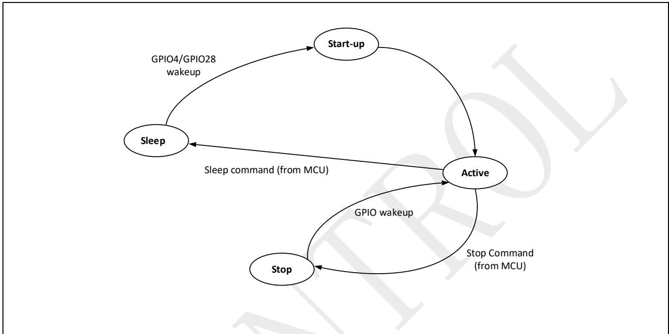
Figure 2-2: Power mode transition
