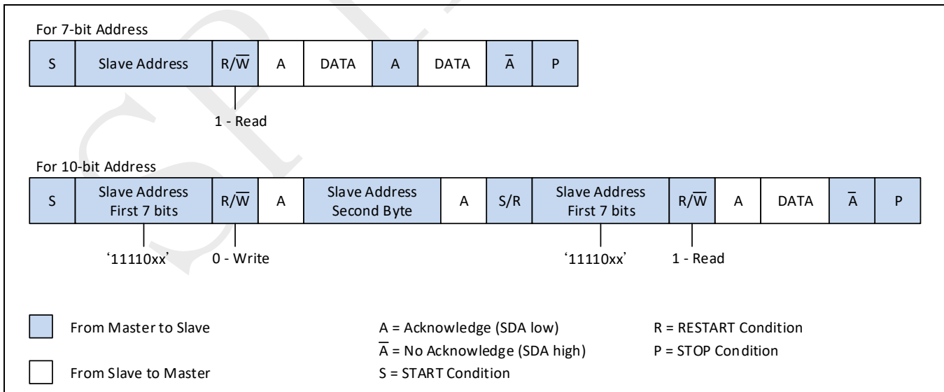
Figure 21-6: Master-receiver protocol
