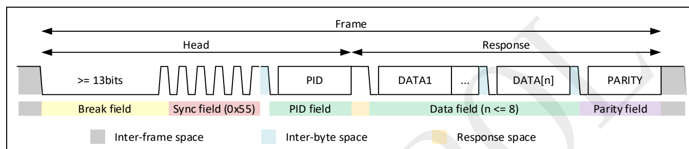
Figure 19-11: LIN frame
