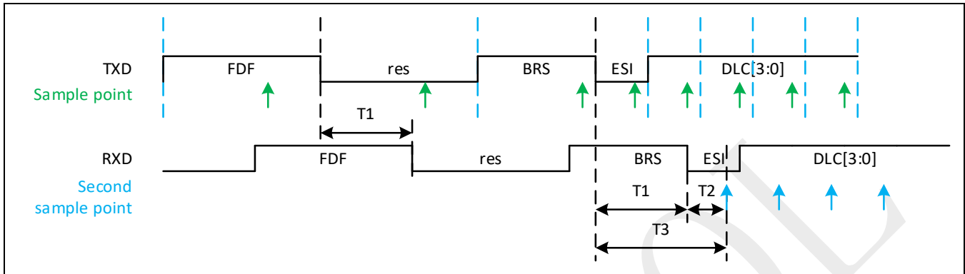
Figure 22-10: Transmitter delay compensation
