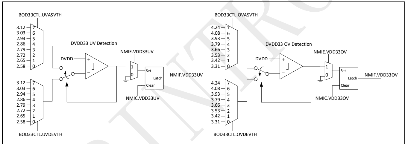
Figure 2-5: 3.3V domain brown-out detector diagram
