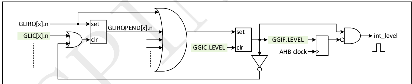
Figure 4-9: GPIO level-triggered interrupt
