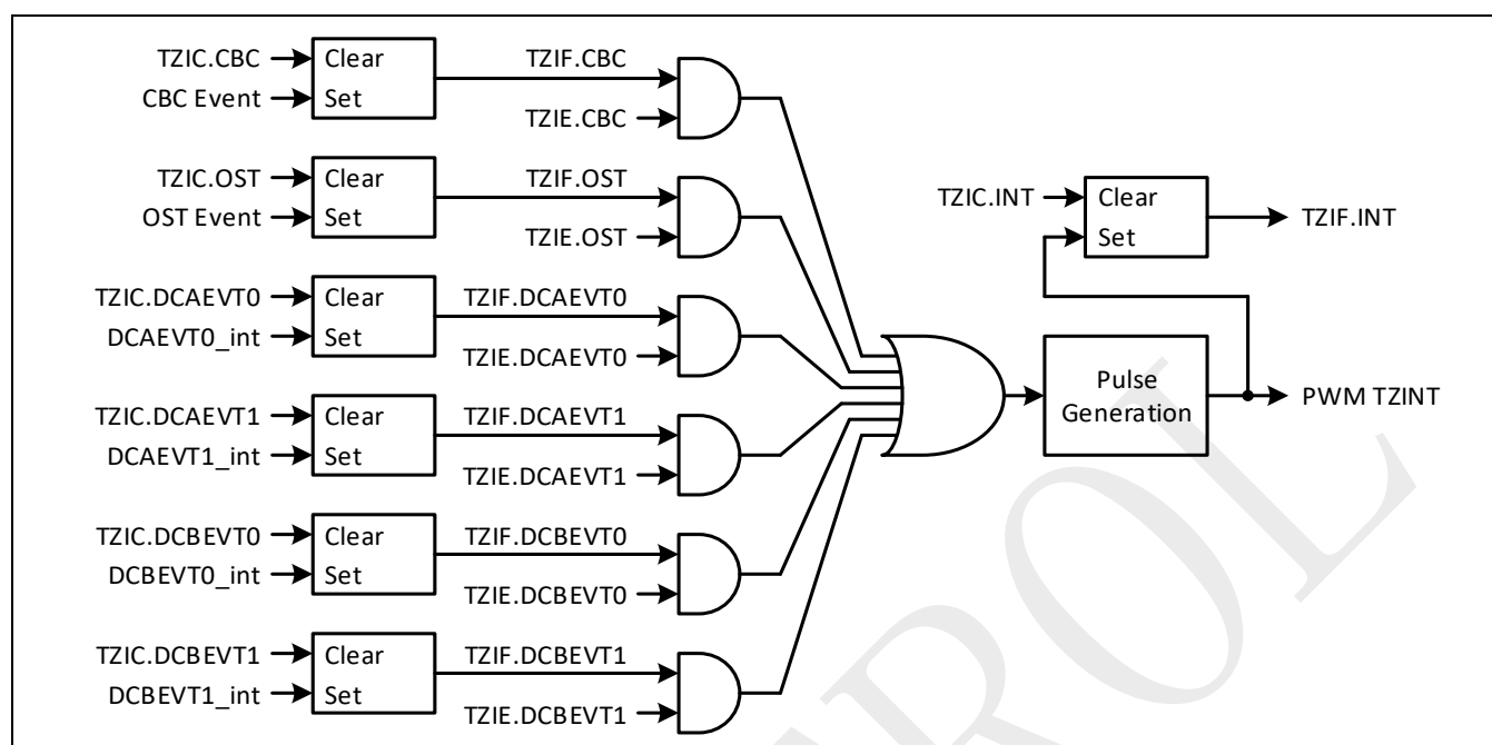
Figure 8-15: Trip-Zone interrupt generation
