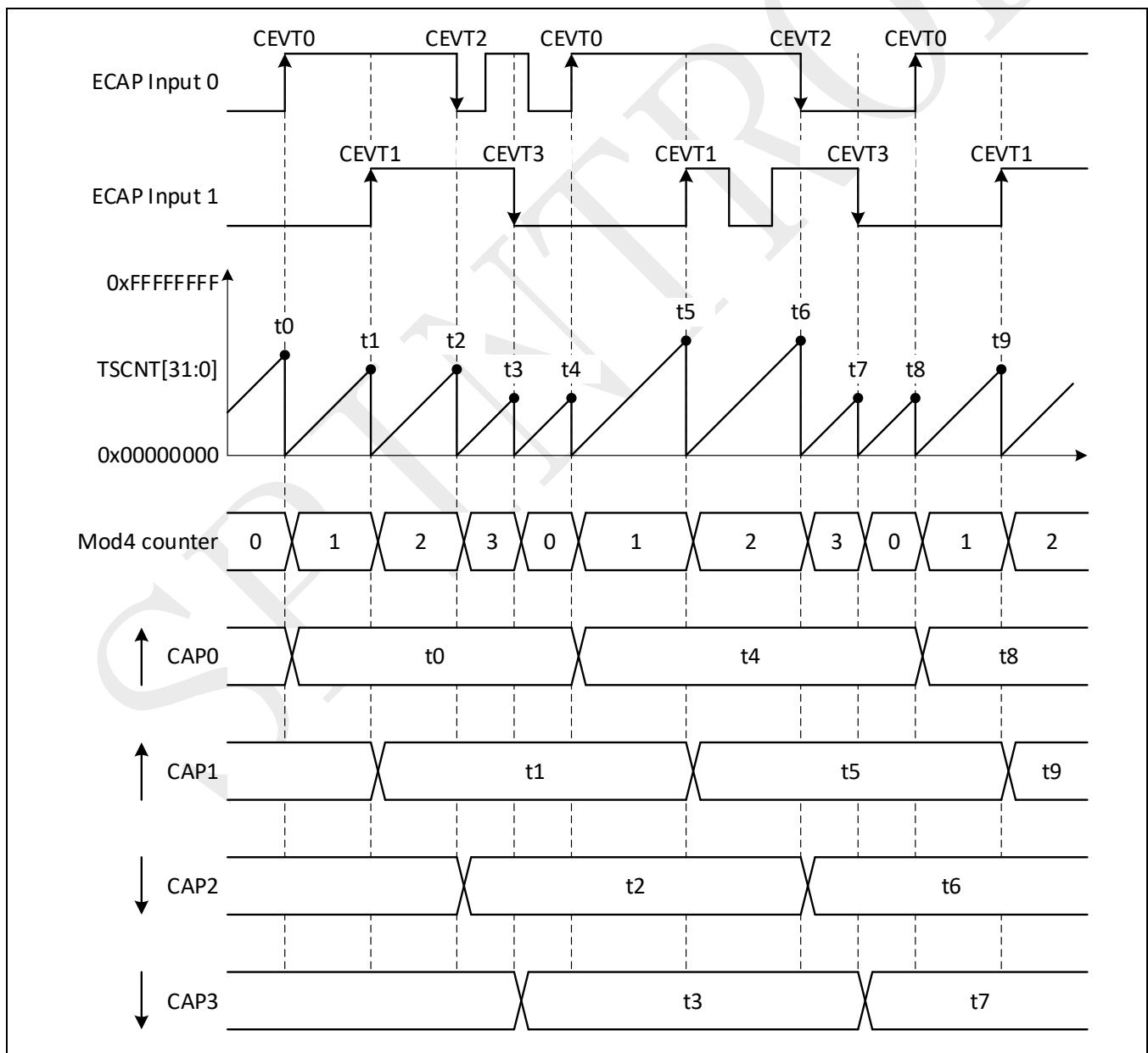
Figure 9-15: Dual pin capture with counter reset
