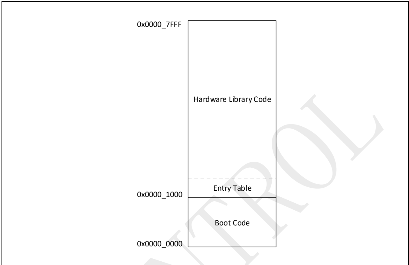
Figure 1-4: Boot ROM memory map
