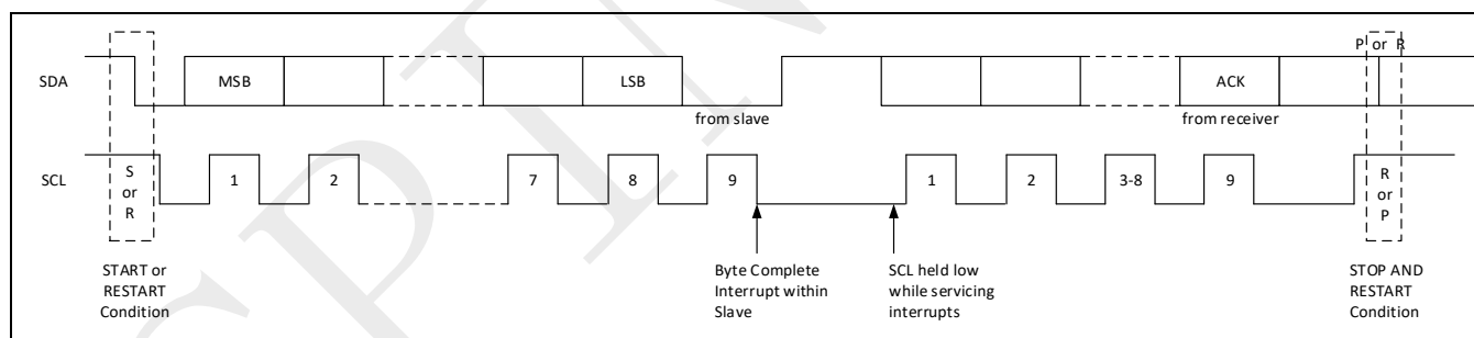
Figure 21-1: Data transfer on the I2C bus
