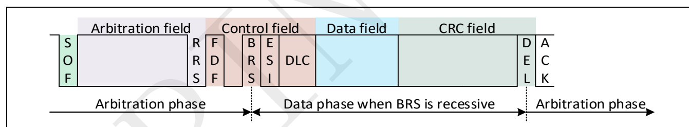
Figure 22-7: Arbitration phase and data phase
