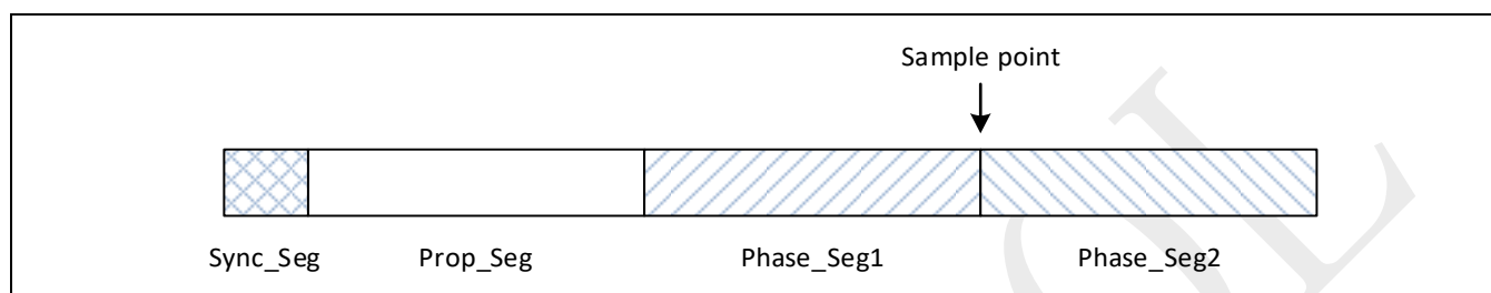
Figure 22-9: Bit timing
