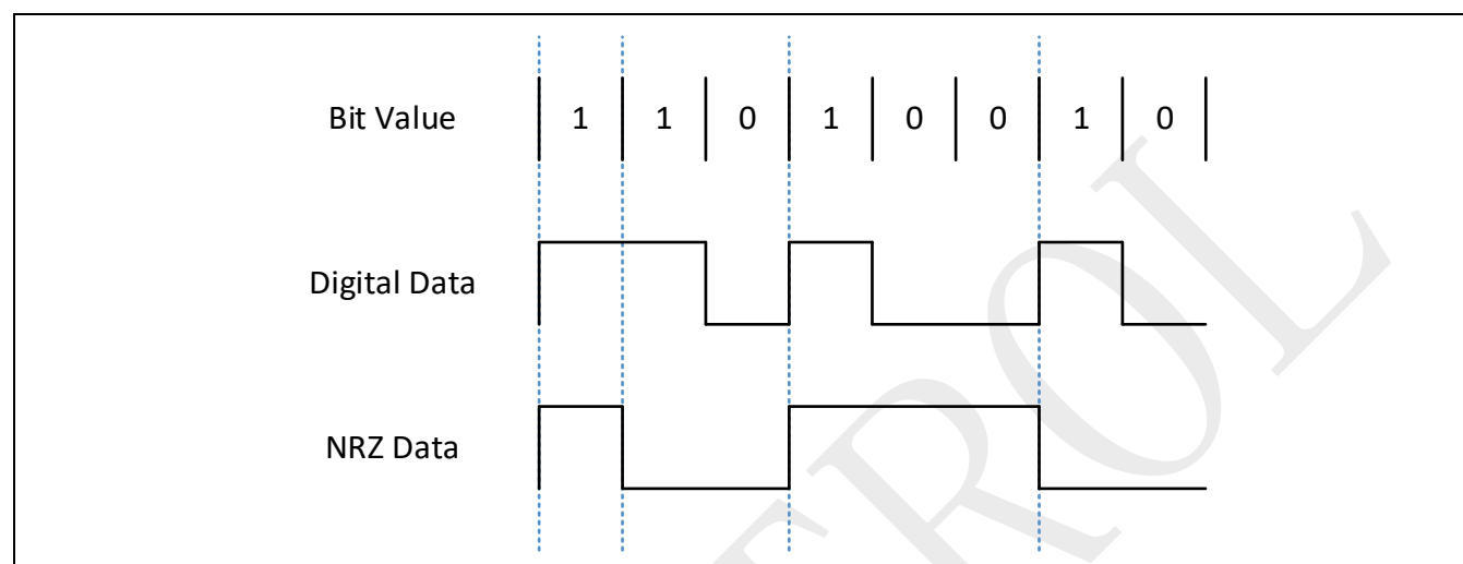
Figure 19-5: Example NRZ bit Encoding – 0b0100_1011
