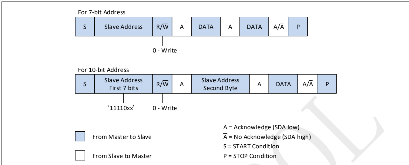
Figure 21-5: Master-transmitter protocol
