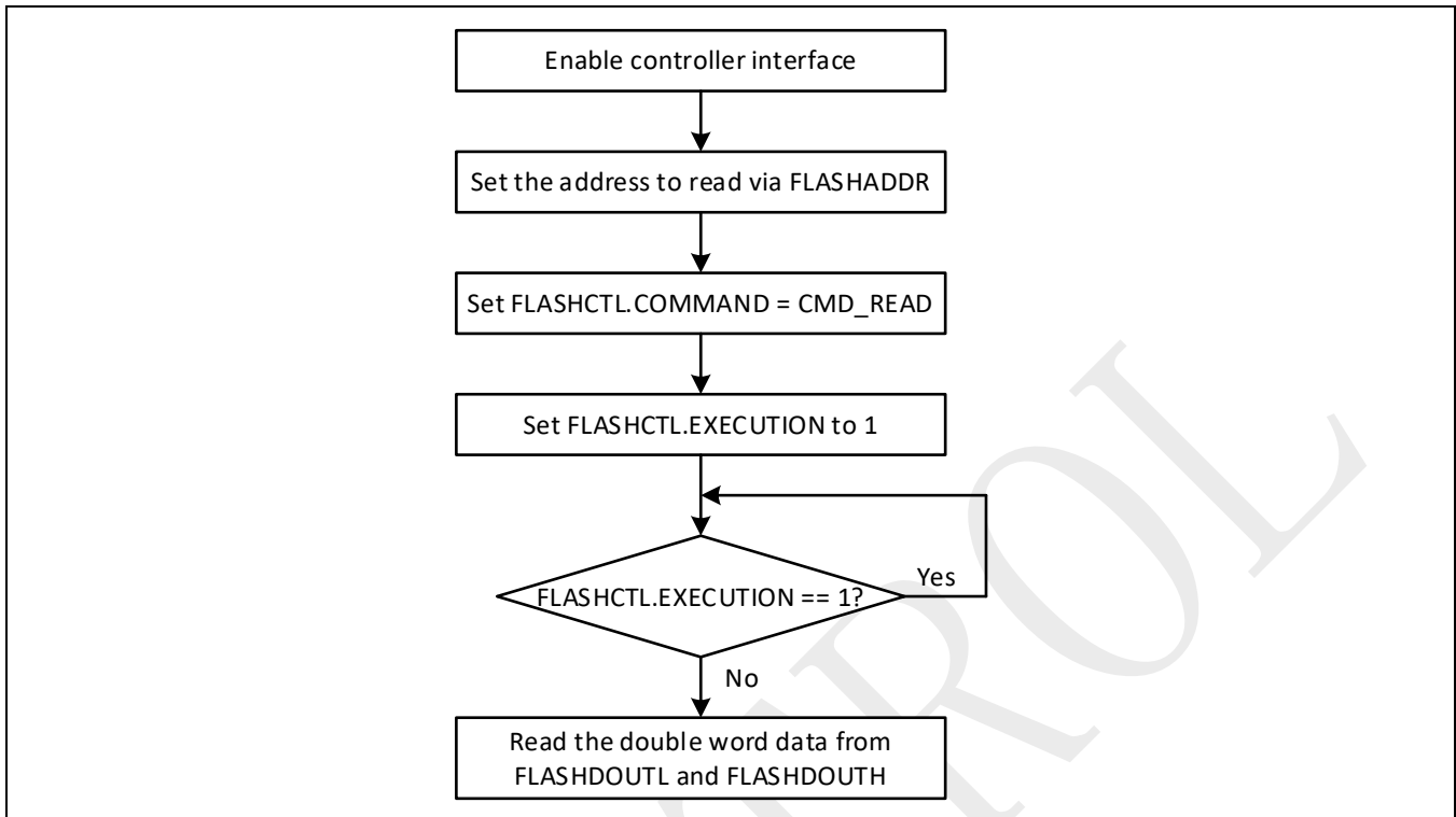
Figure 24-3: Flash memory reading procedure
