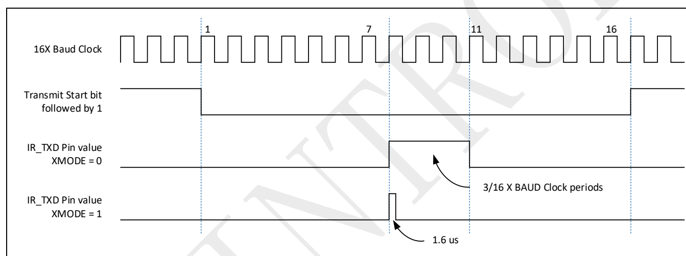
Figure 19-8: XMODE example
