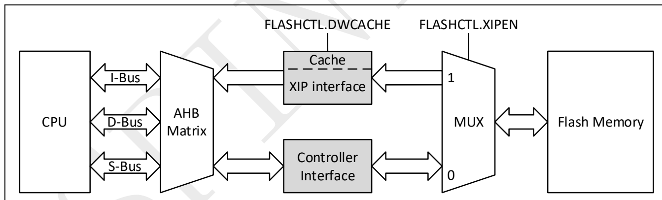
Figure 24-1: Flash memory access interfaces
