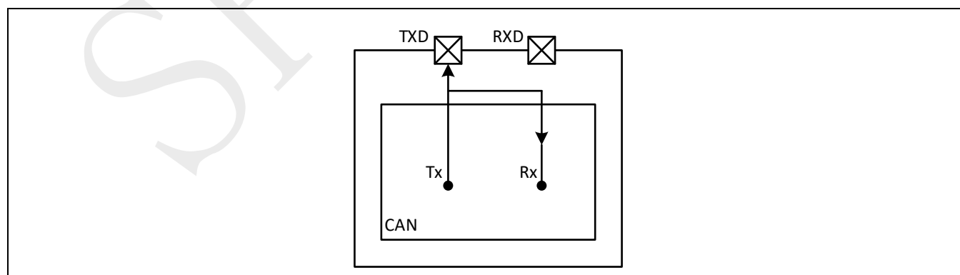
Figure 22-13: External loopback mode
