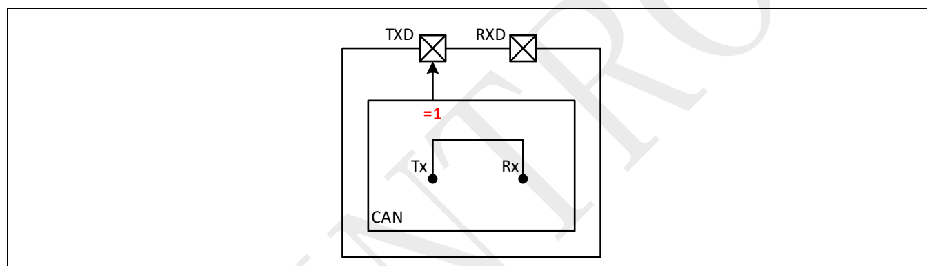
Figure 22-12: Loopback mode
