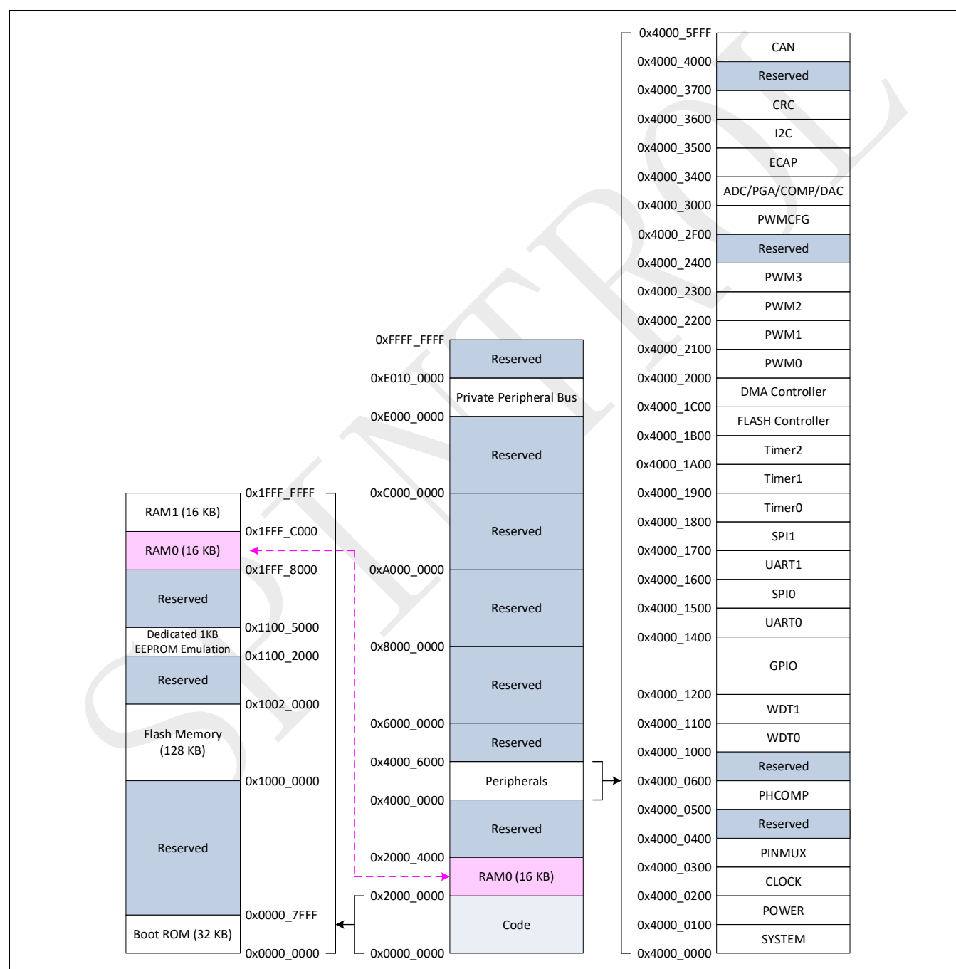
Figure 1-3: SPC1169 memory map
