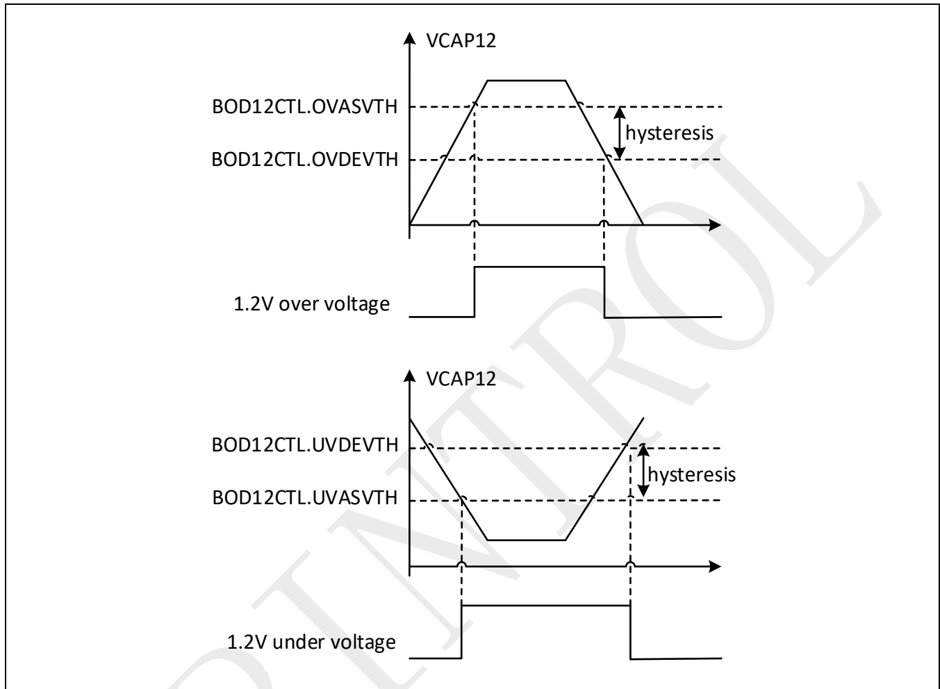
Figure 2-8: VCAP12 thresholds
