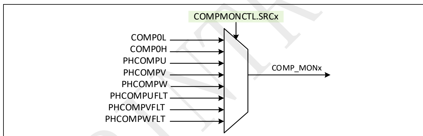
Figure 4-4: Select source of COMP_MONx
