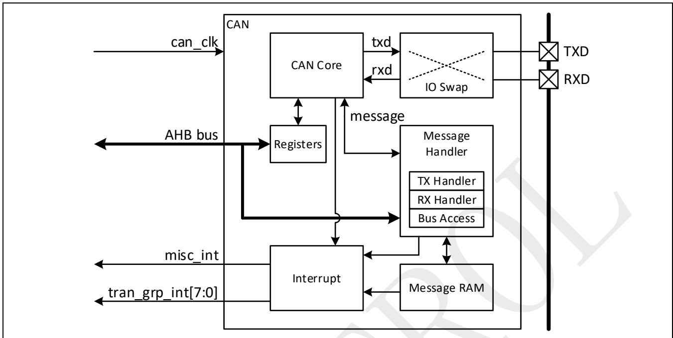
Figure 22-1: CAN Block Diagram
