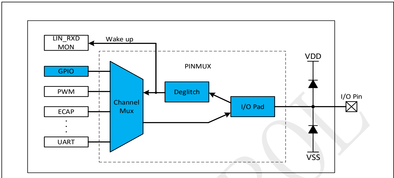
Figure 4-1: Block diagram of I/O control
