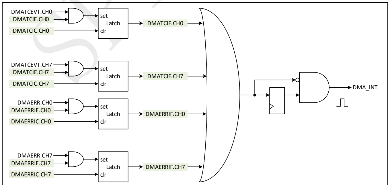
Figure 26-4: DMA interrupt generation
