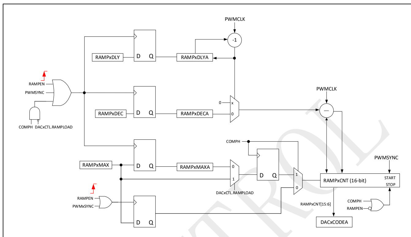
Figure 16-2: Ramp generator diagram
