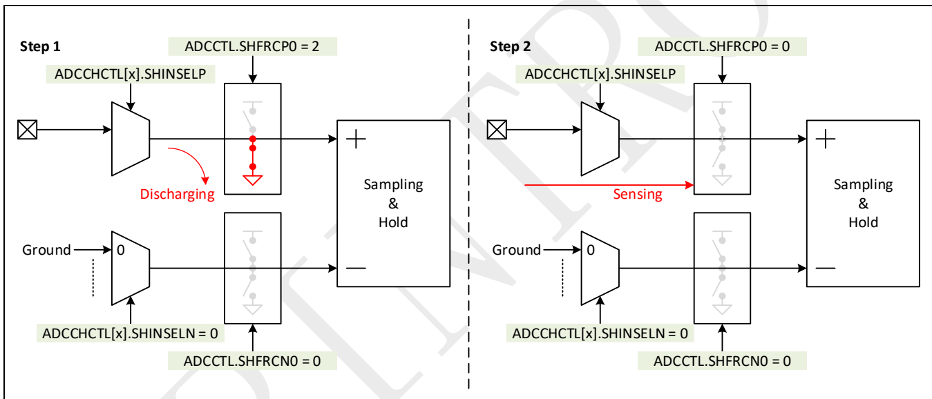
Figure 10-11: Detect the pin floating of ADC input (fault injection by precharging)
