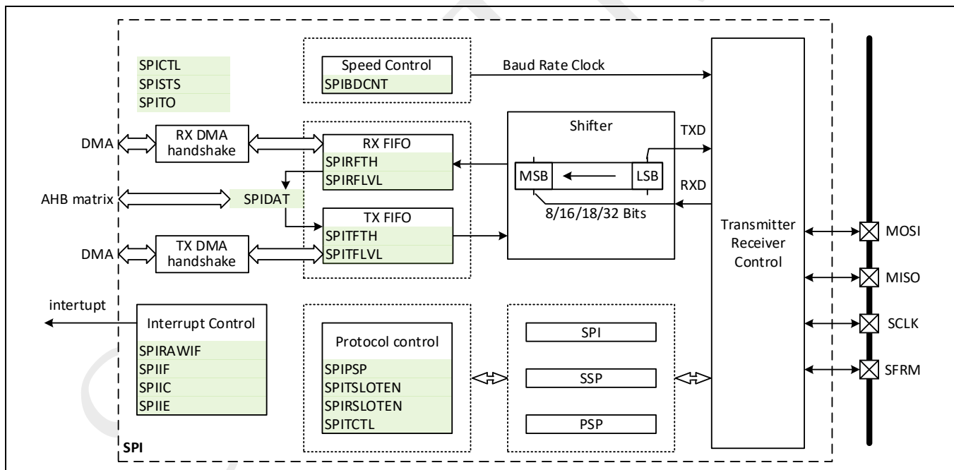
Figure 20-1: SPI block diagram
