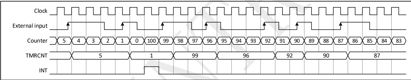
Figure 6-5: Timer waveform in event capture mode (TMRLOAD=100)
