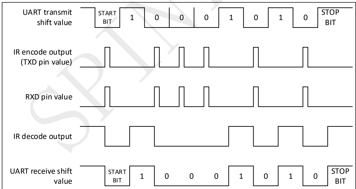
Figure 19-7: IR transmit and receive example
