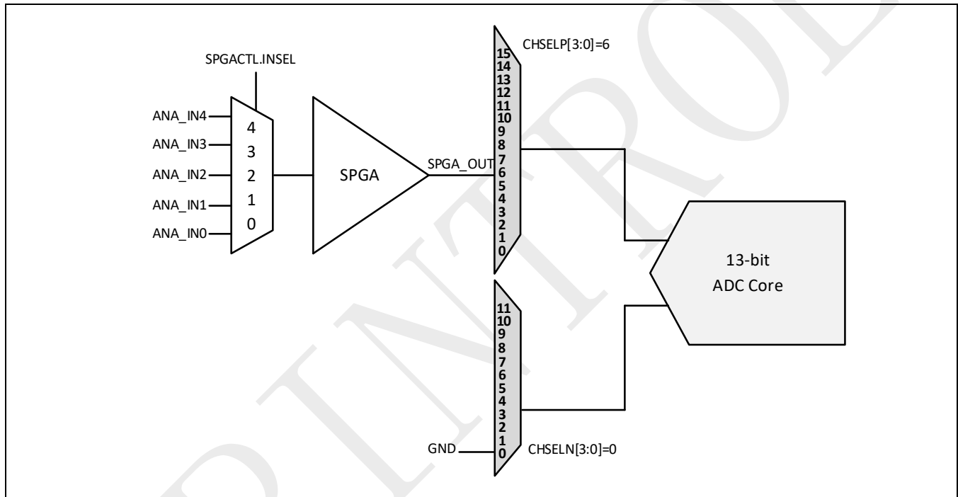
Figure 12-1: SPGA block architecture
