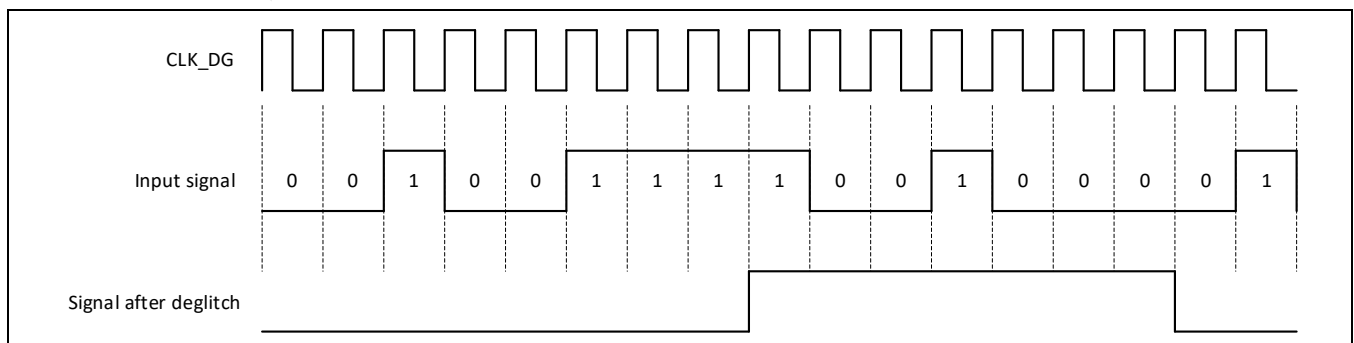
Figure 4-3: Input deglitching
