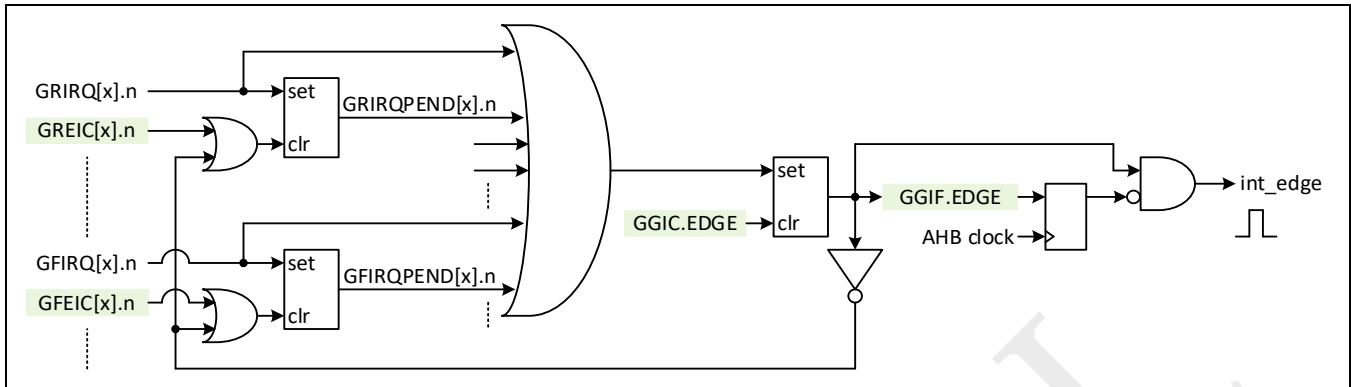
Figure 4-7: GPIO edge-triggered interrupt
