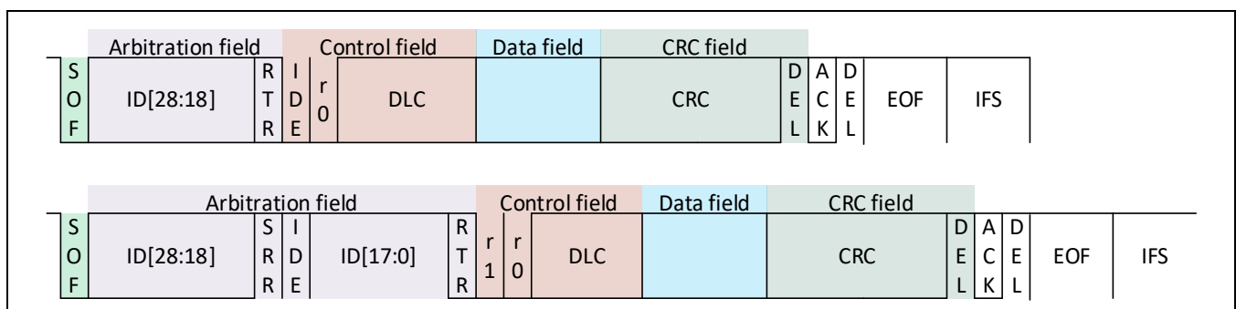
Figure 22-5: CAN2.0B CAN frame format
