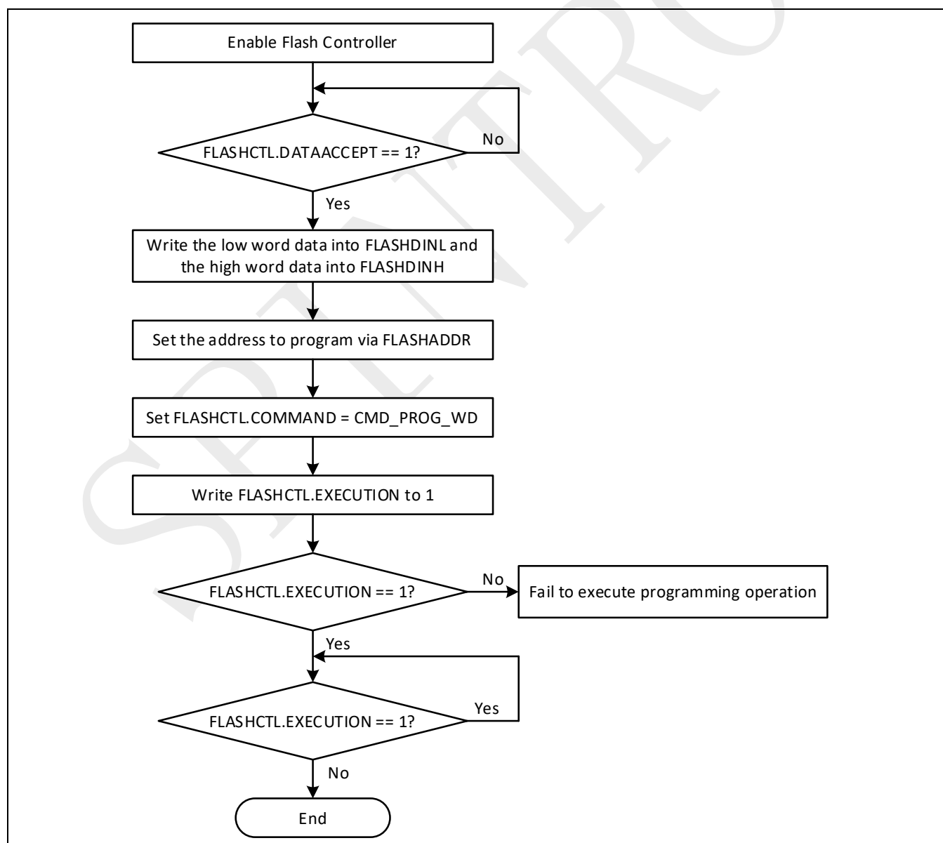
Figure 24-4: Flash memory programming procedure
