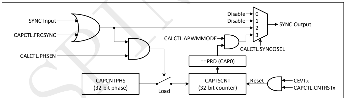
Figure 9-7: Details of the counter and synchronization block
