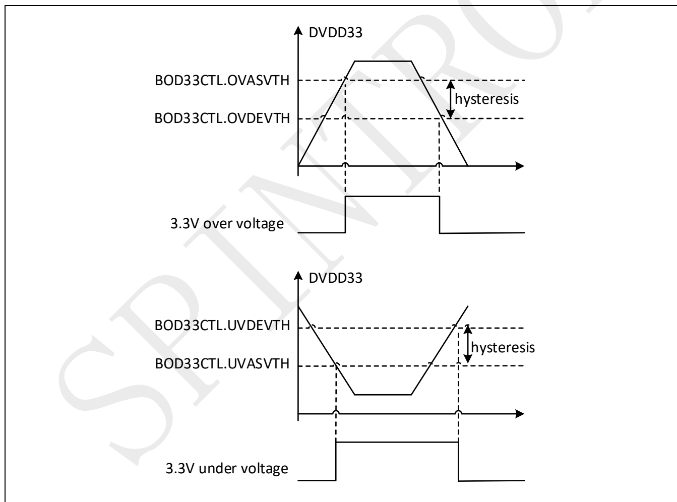
Figure 2-7: DVDD33 thresholds
