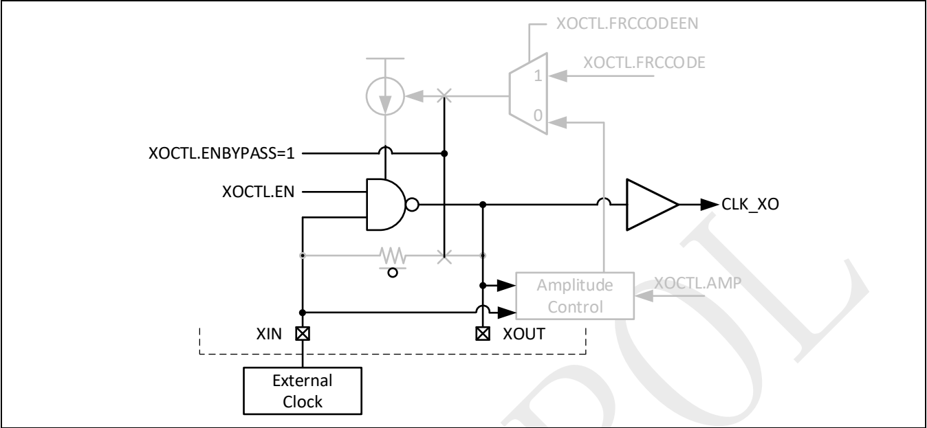
Figure 3-5: External clock
