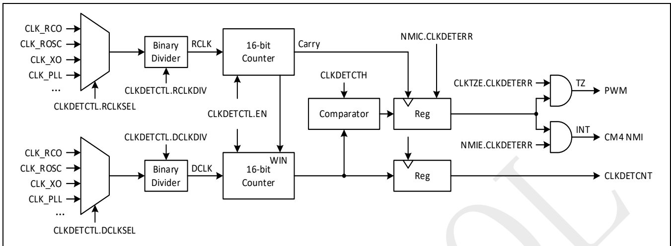
Figure 3-8: Clock cross-detection
