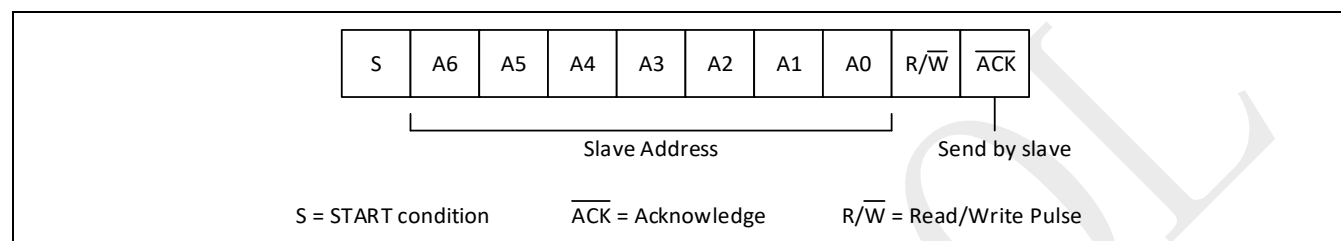
Figure 21-3: 7-bit address format
