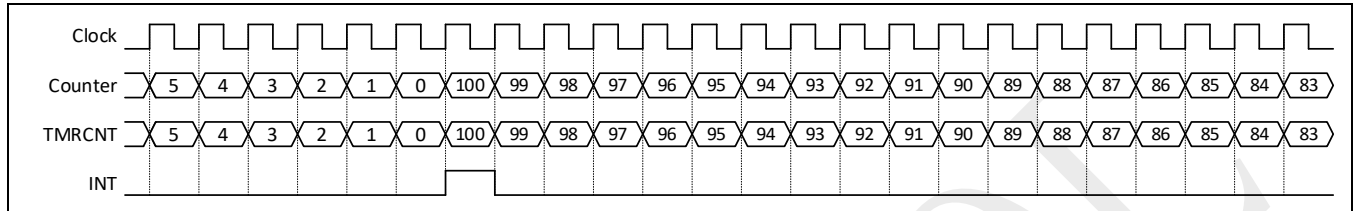
Figure 6-2: Timer waveform in general timer mode (TMRLOAD=100)
