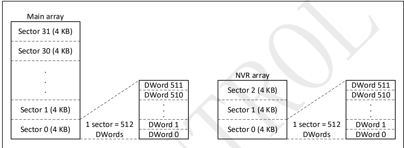
Figure 24-2: Logical structure of the Flash module
