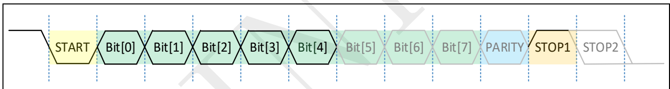
Figure 19-4: UART frame
