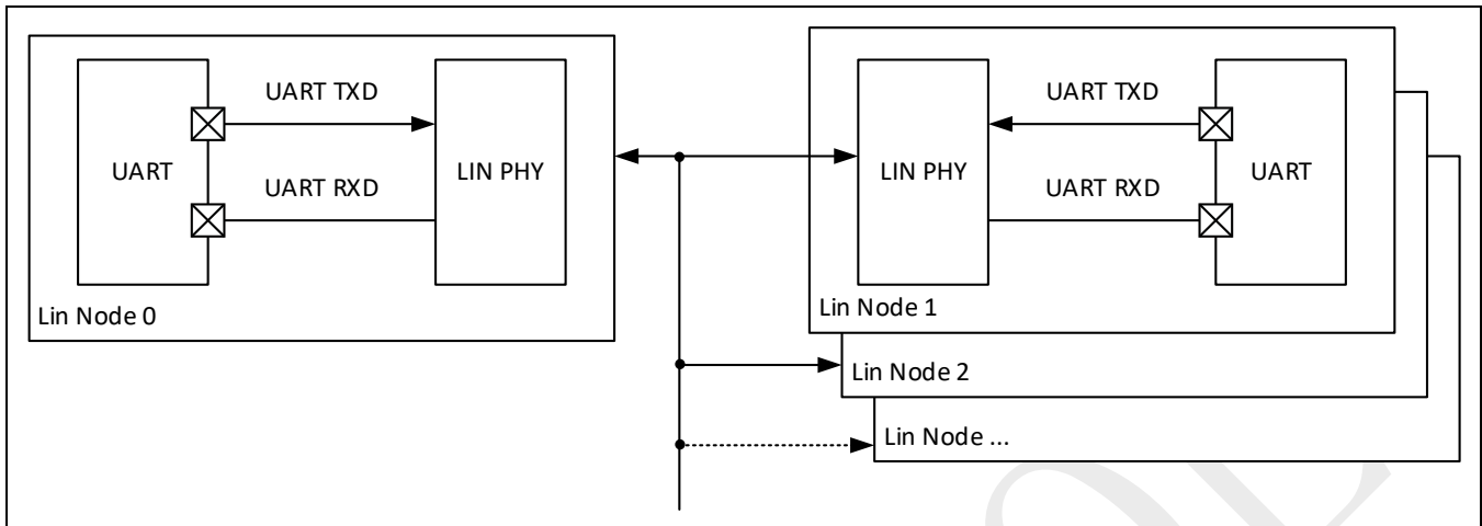
Figure 19-3: UART LIN device connection diagram
