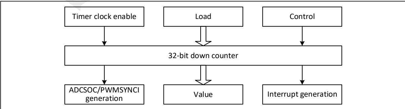
Figure 6-6: GPT run flow diagram
