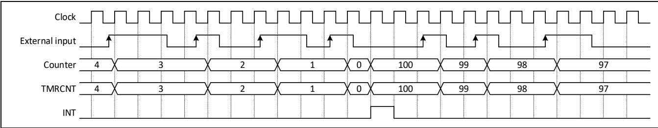
Figure 6-4: Timer waveform in event counter mode (TMRLOAD=100)
