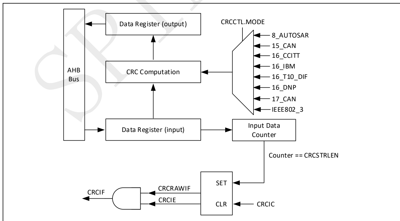
Figure 23-1: CRC block diagram
