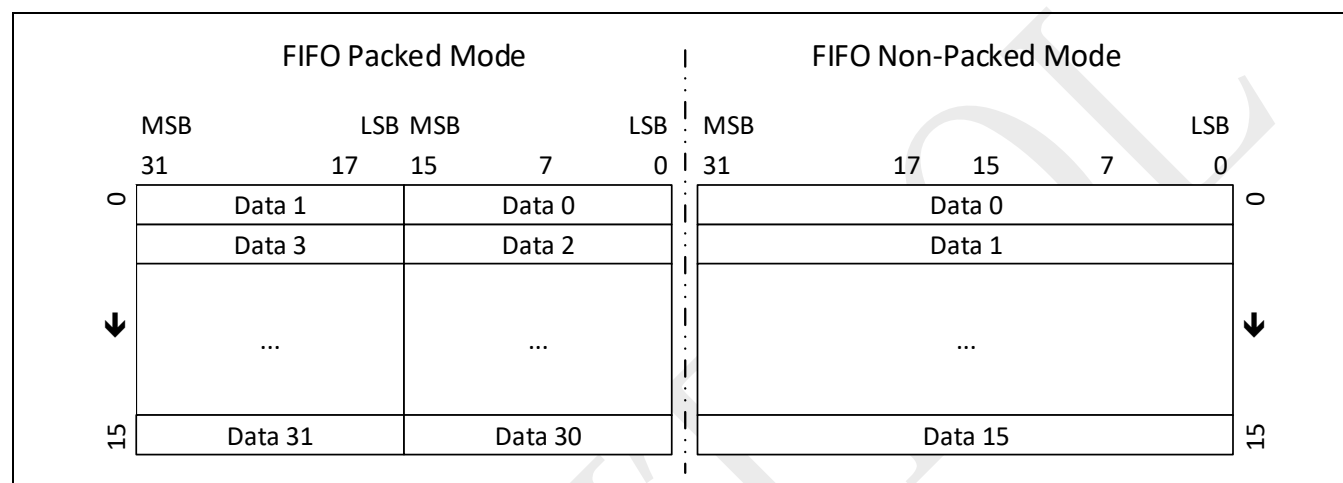
Figure 20-2: FIFO packed and non-packed mode
