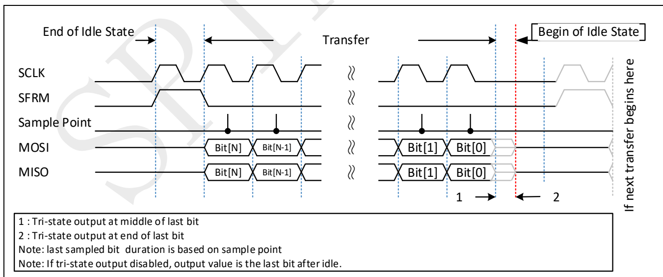
Figure 20-7: SSP protocol (single transfer)
