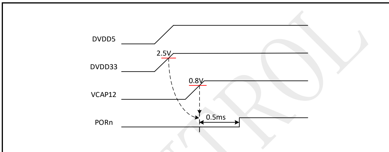
Figure 2-3: Power up sequence
