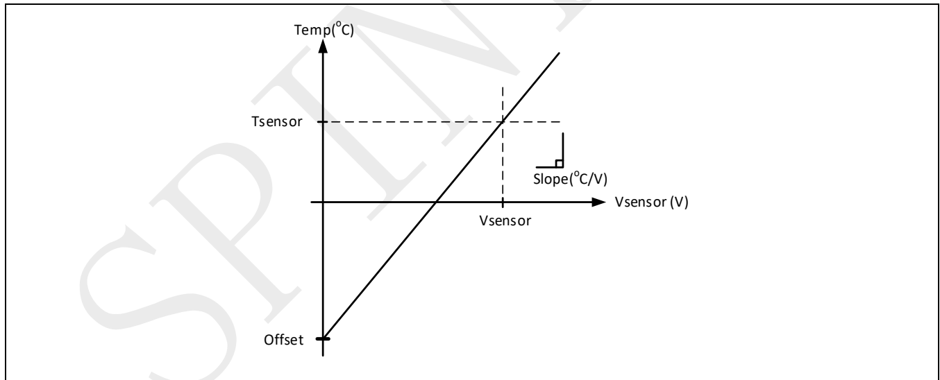
Figure 18-1: Temperature sensor transfer function
