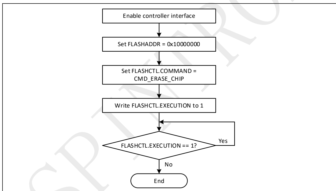
Figure 24-6: Flash memory Chip Erase procedure
