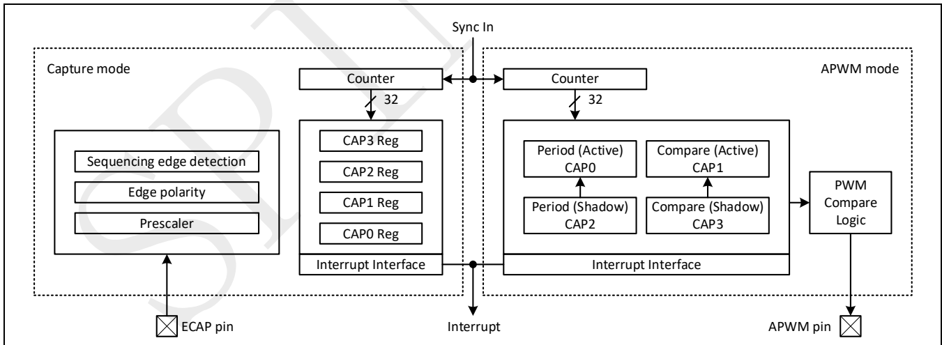
Figure 9-2: Capture and APWM modes of operation
