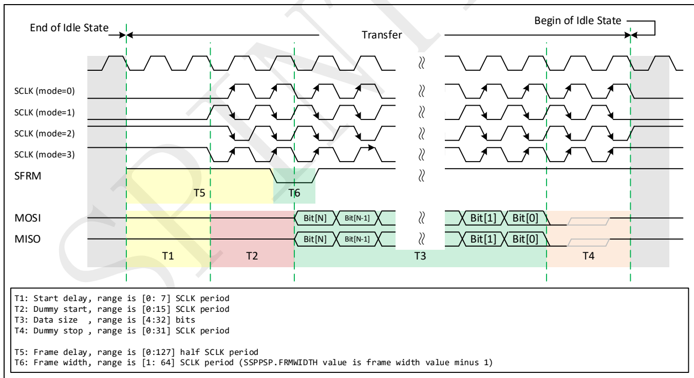
Figure 20-9: PSP protocol (single transfer)
