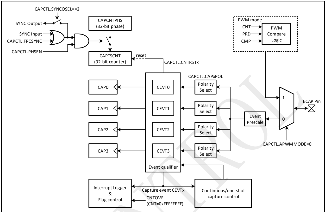
Figure 9-3: Capture function diagram
