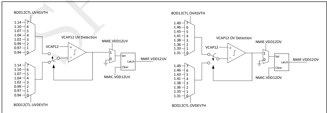
Figure 2-6: 1.2V domain brown-out detector diagram
