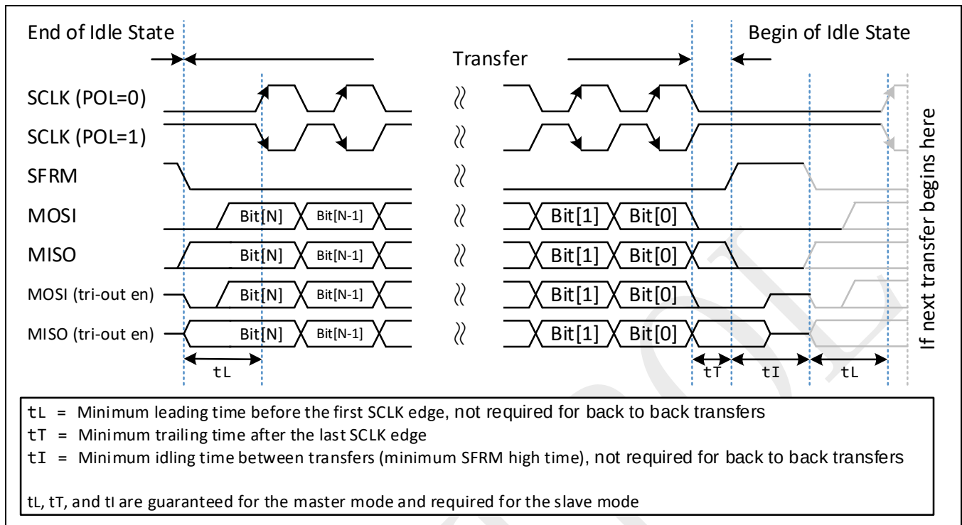
Figure 20-4: SPI protocol (PHS = 0)
