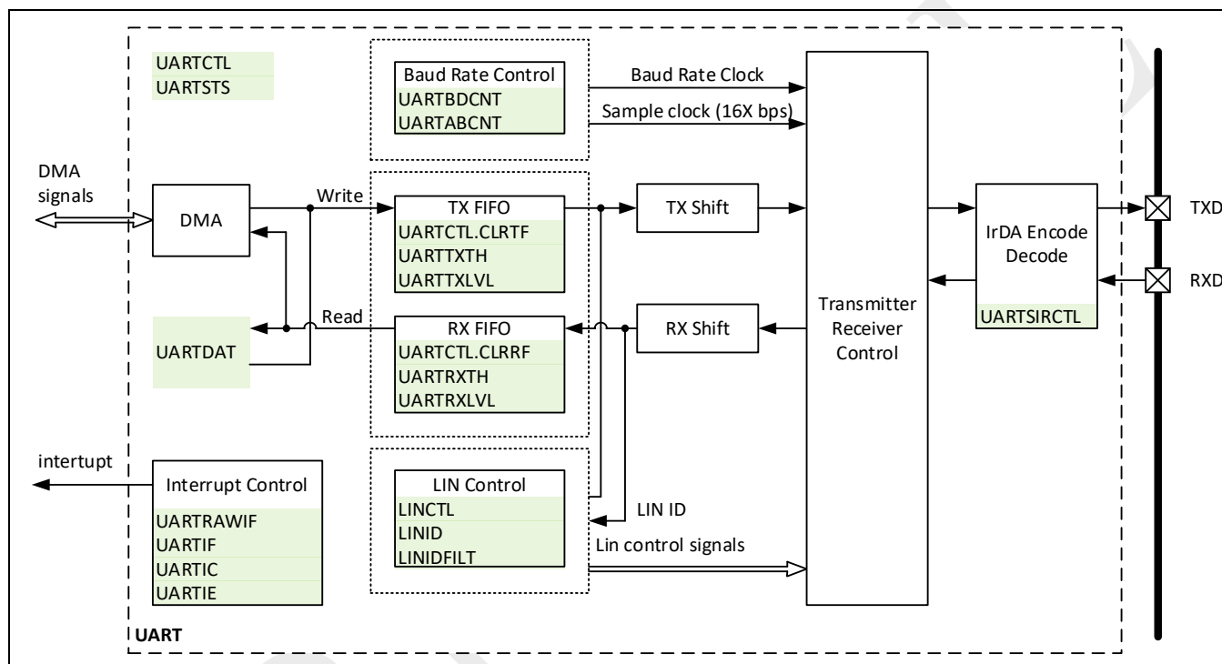
Figure 19-1: UART block diagram
