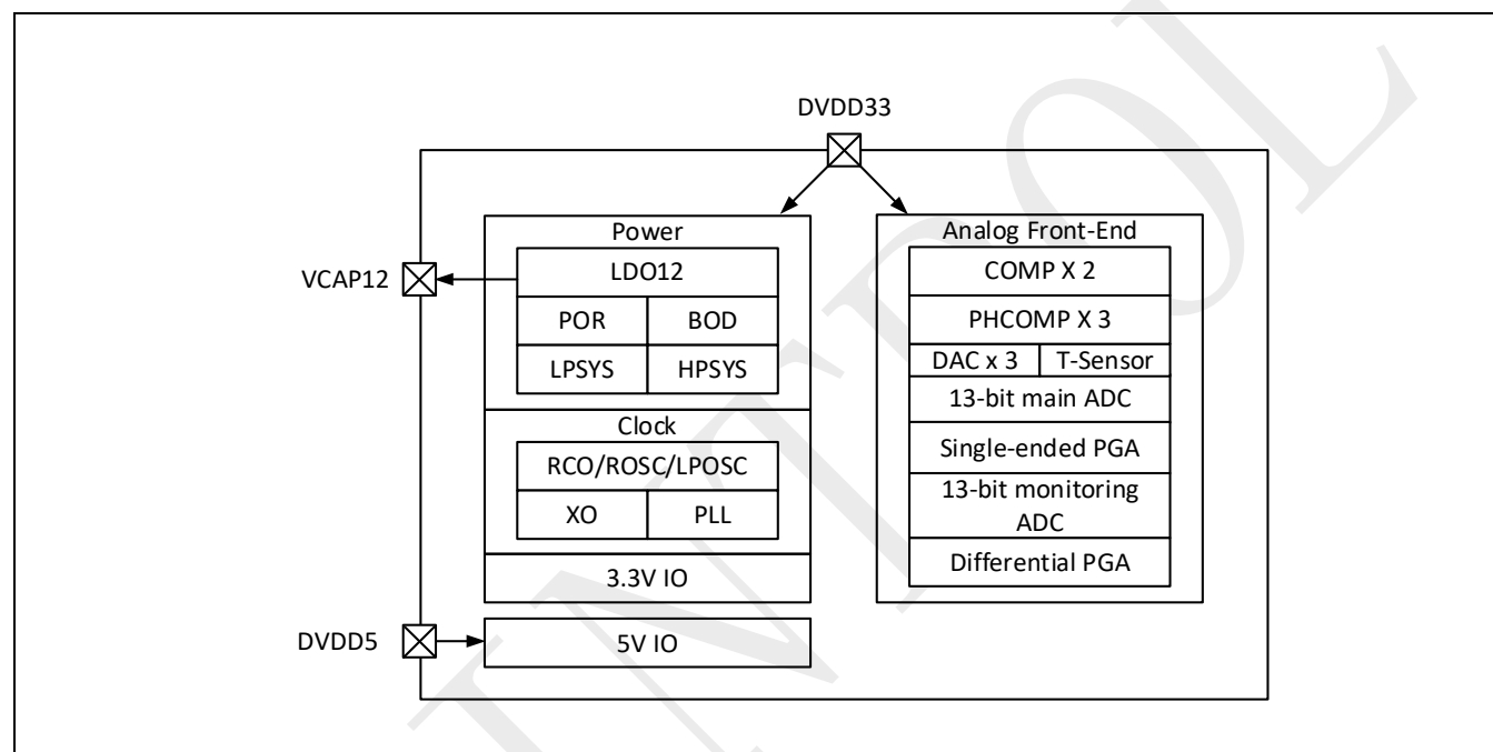
Figure 2-1: Power supply overview
