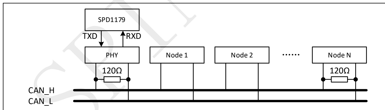
Figure 22-2: CAN device connection
