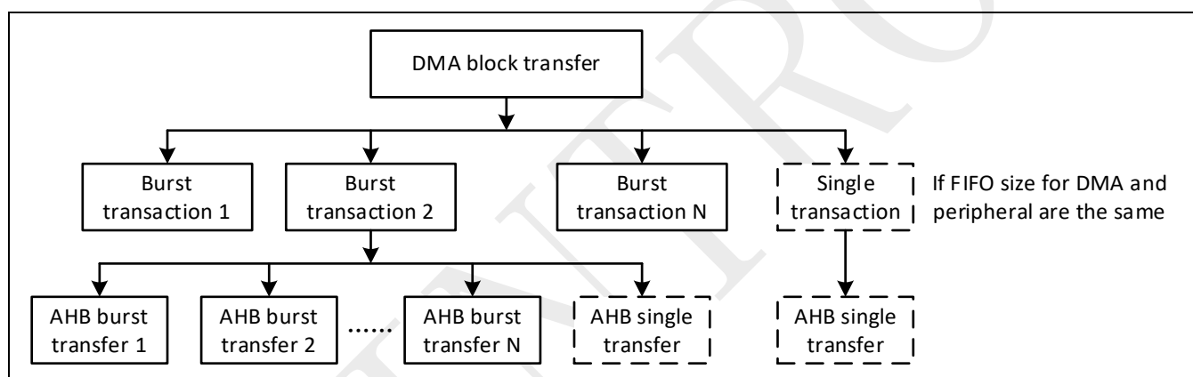
Figure 26-3: Breakdown of DMA transfer for non-memory peripherals
