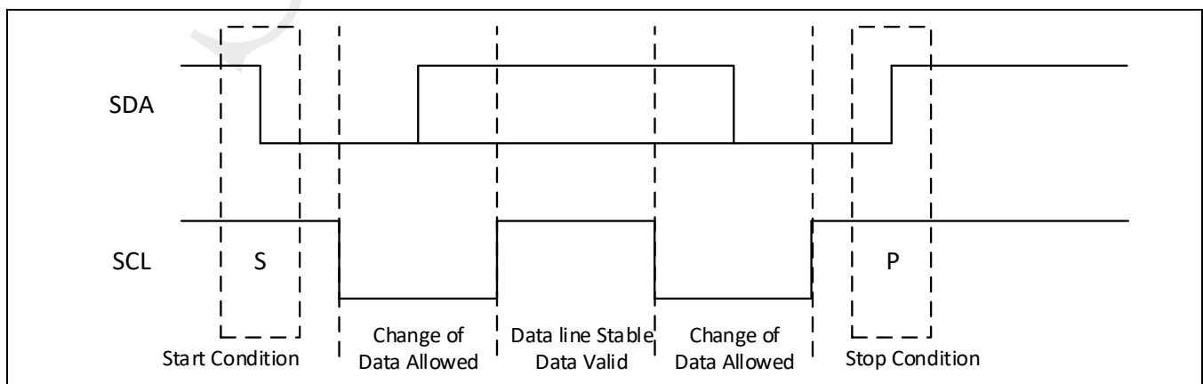
Figure 21-2: START and STOP condition
