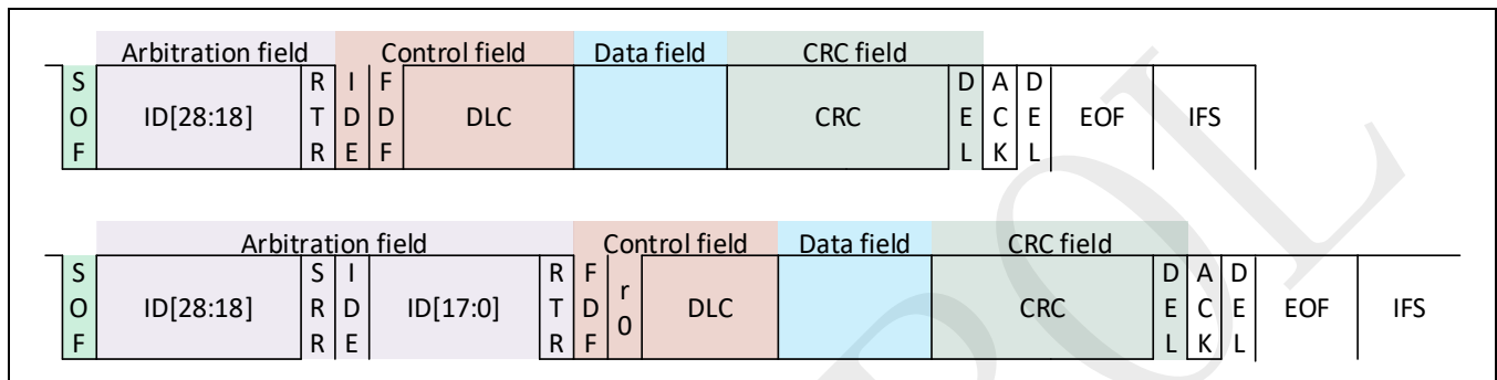
Figure 22-3: ISO classical CAN frame format
