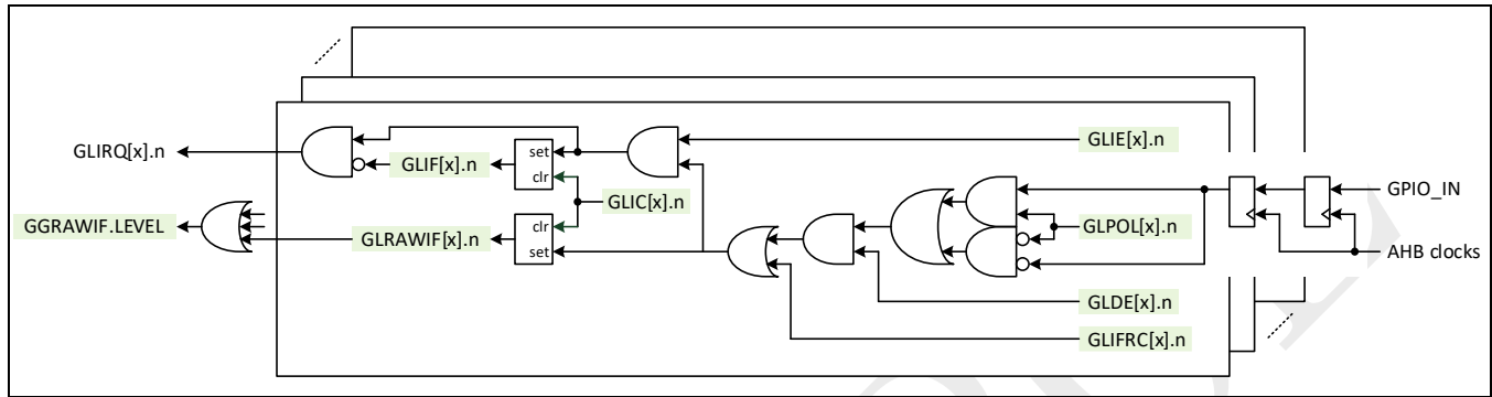
Figure 4-8: GPIO level detect
