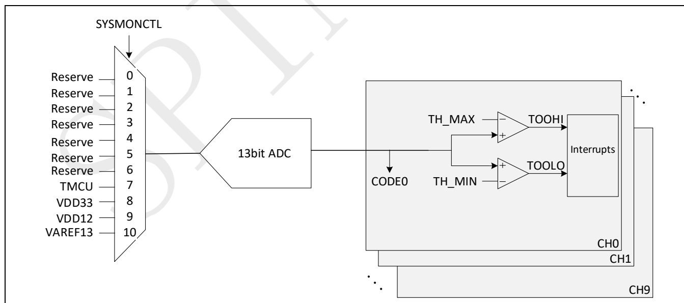
Figure 11-1: 13-bit Monitoring ADC block diagram
