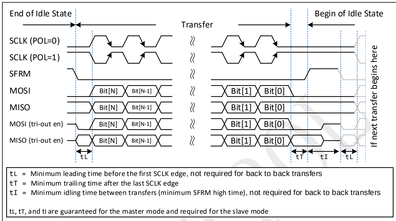
Figure 20-5: SPI protocol (PHS = 1)
