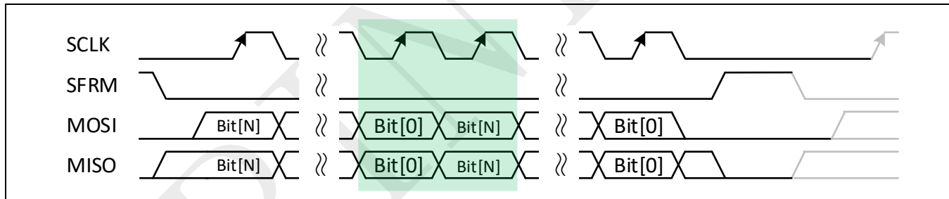
Figure 20-6: SPI protocol (back to back transfer)
