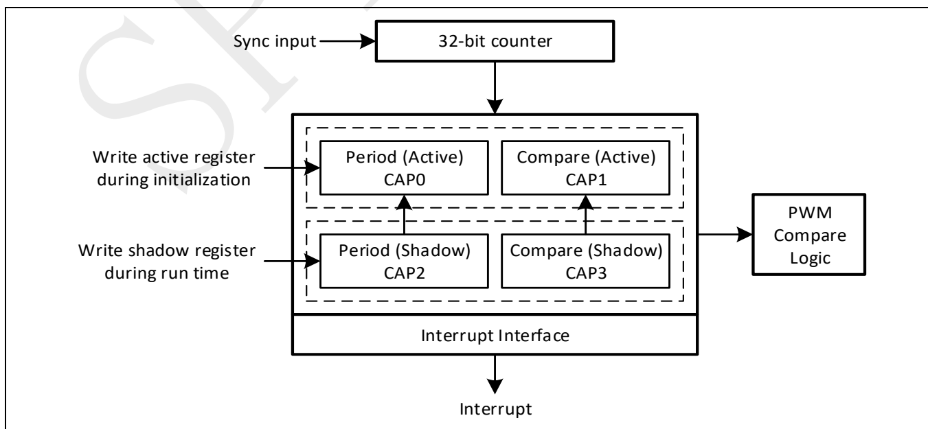
Figure 9-9: Active and shadow register in APWM mode
