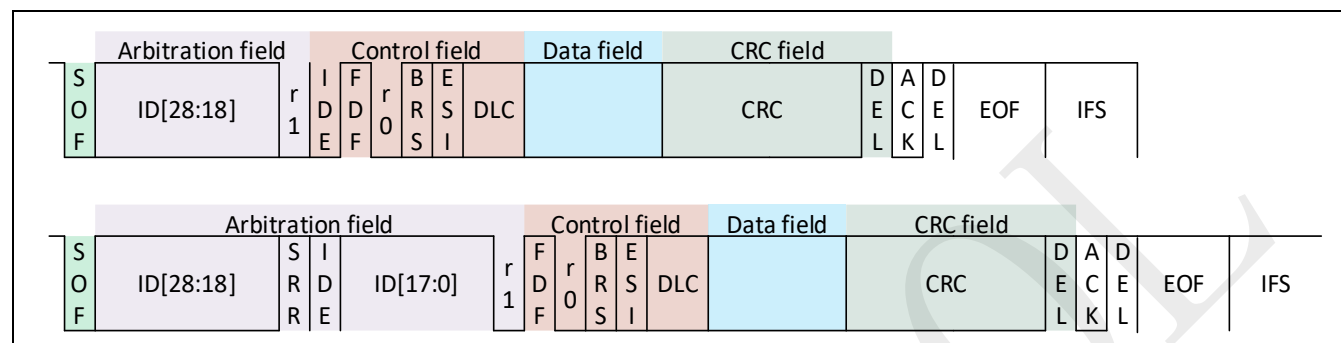
Figure 22-6: NONISO FDCAN frame format
