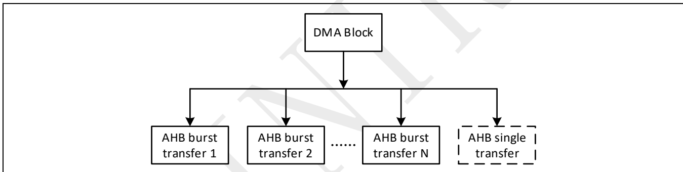
Figure 26-2: Breakdown of DMA transfer for memory
