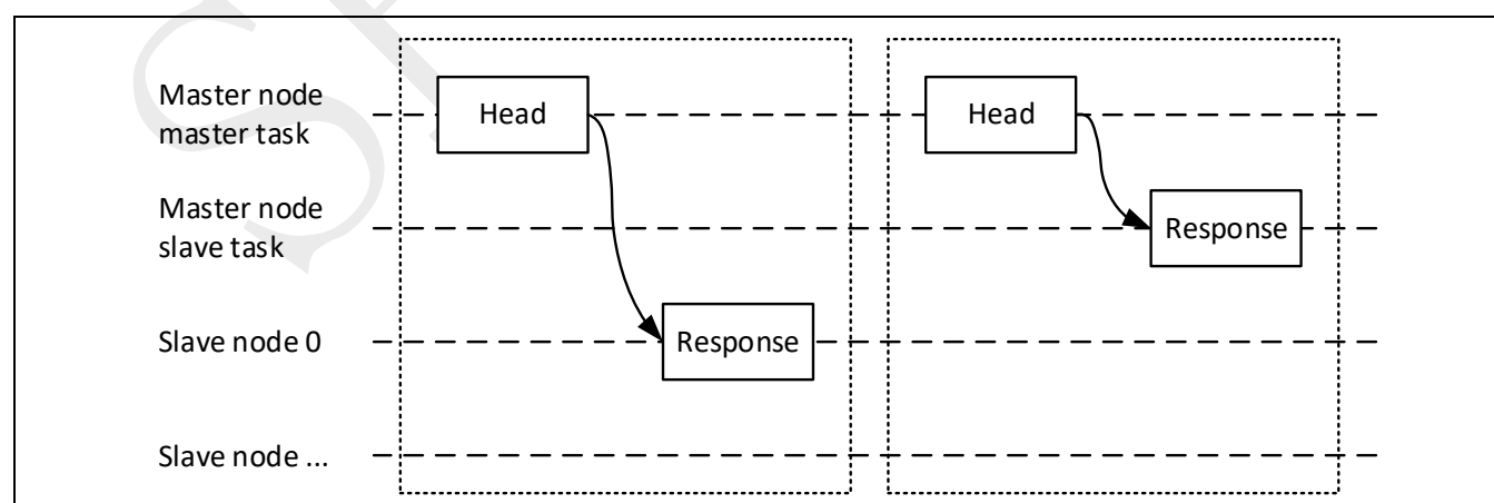
Figure 19-12: LIN transfer
