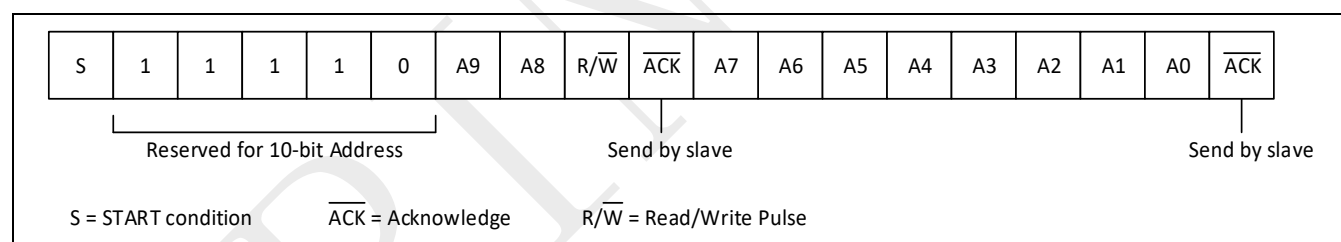
Figure 21-4: 10-bit address format
