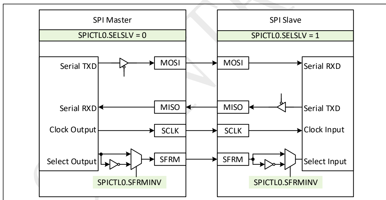
Figure 20-3: SPI master-slave connection
