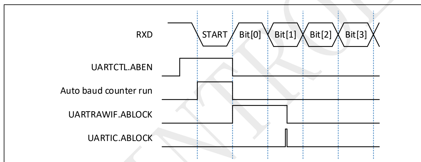
Figure 19-6: Example of auto baud
