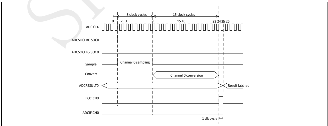
Figure 10-5: Timing example
