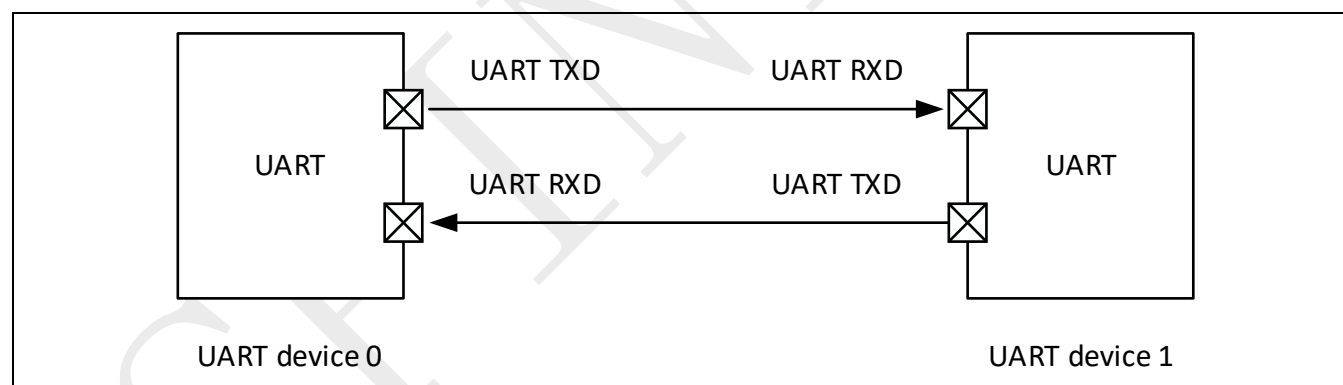
Figure 19-2: UART device connection diagram
