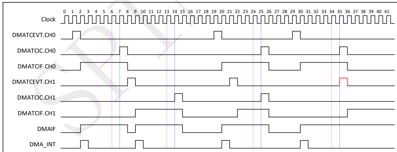
Figure 26-6: Scenario DMA interrupt events for multiple channels
