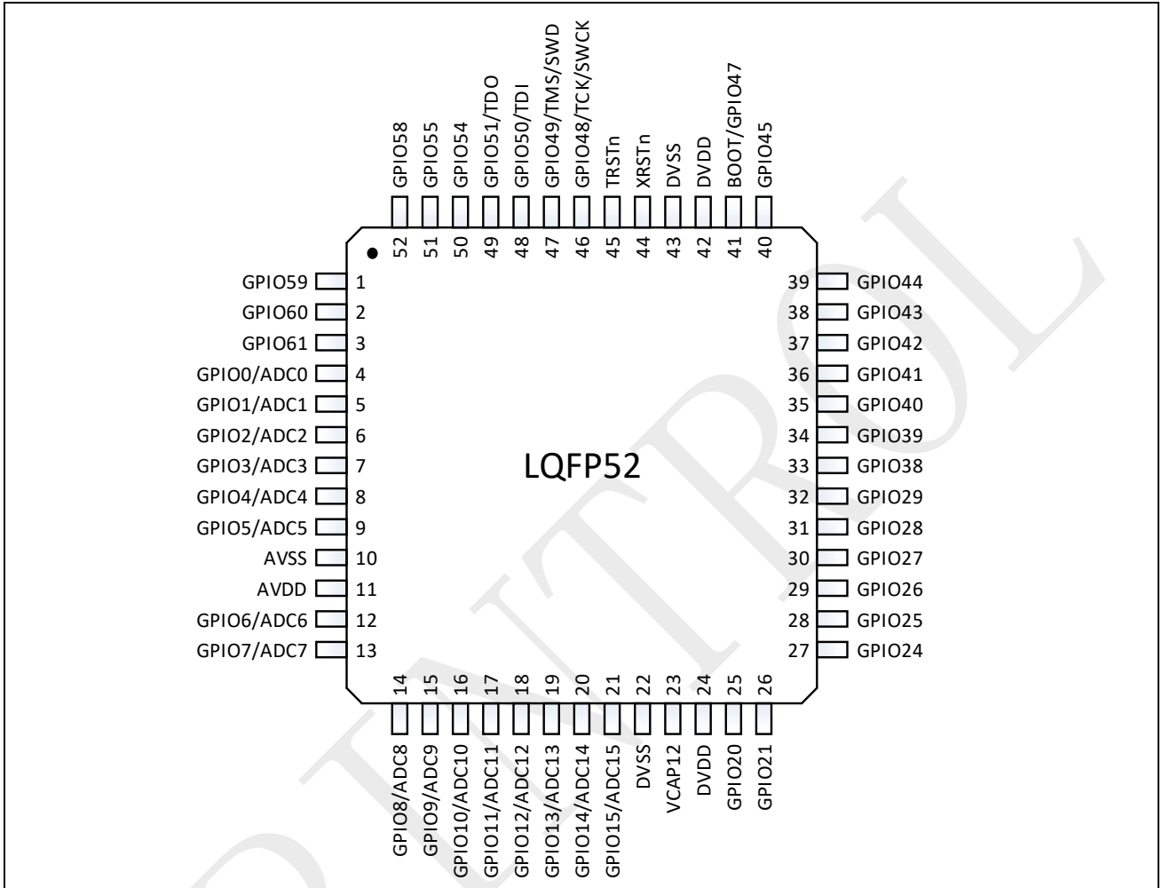
图 3-3: SPC1198 LQFP52 引脚排列
